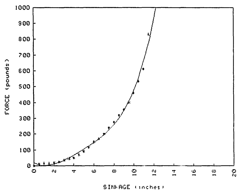
Figure 4. Exponential curve fit on plate-sinkage data.
