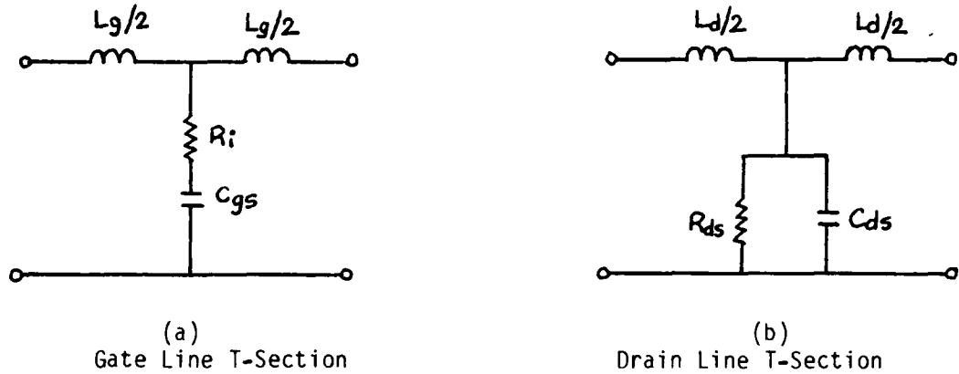
Fig. 2. Gate and drain line T-sections.
