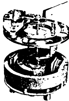
Figure 3.1 Interior View of Iron-cored Dynamometer Wattmeter Movement
