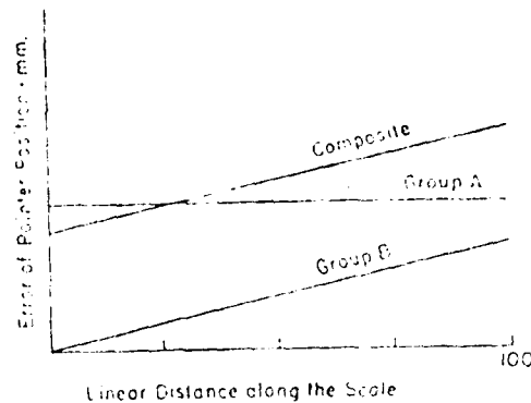
Figure 5.1 Curves Showing Variation Along the Scale of Various Types of Instrument Error
