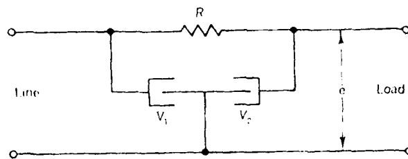
Figure 3.2 Electrostatic Wattmeter
