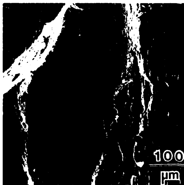
Figure 20. SEM observations within the split regions. All observations indicate fracture was ductile in nature.
