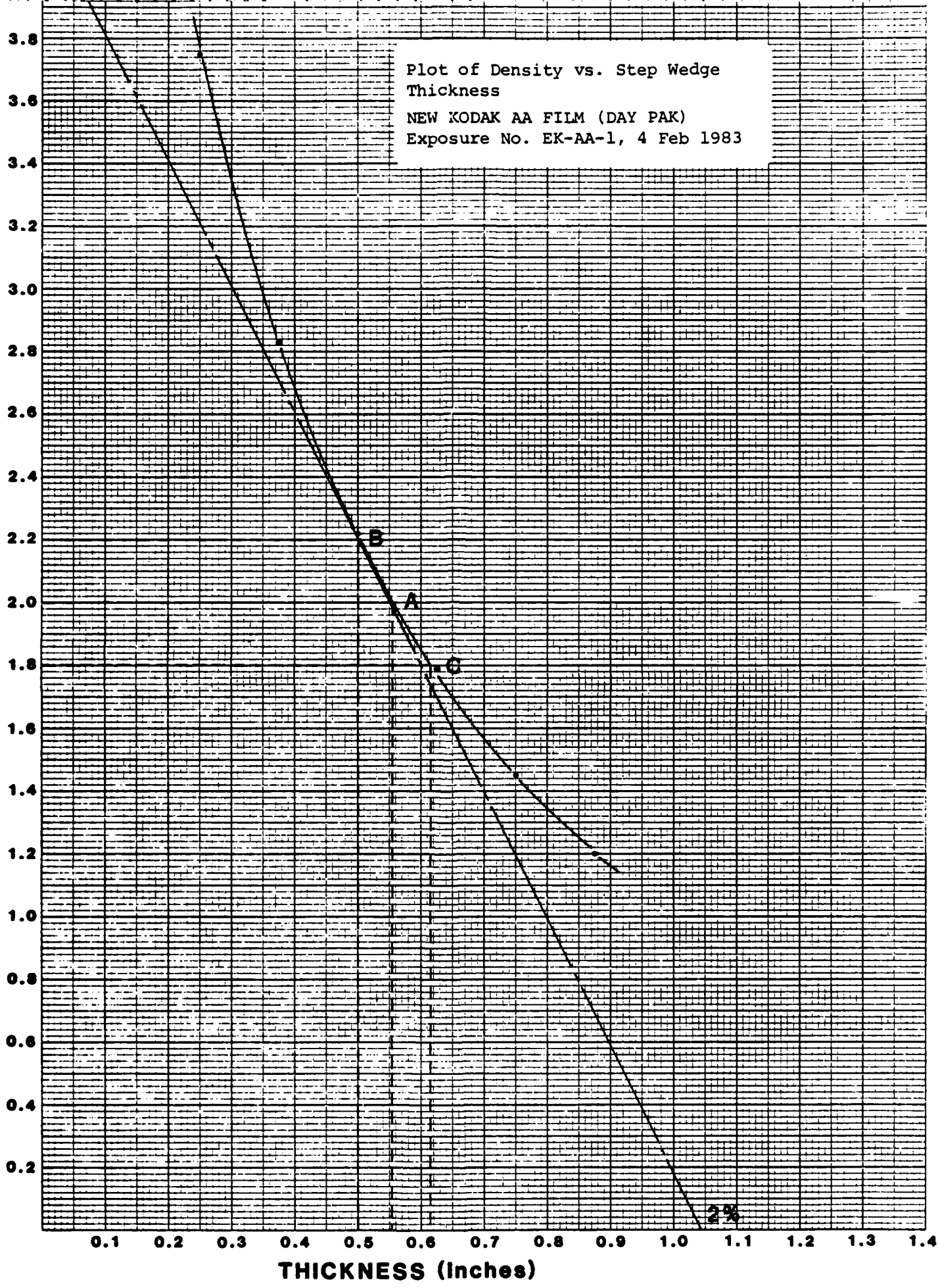
FIGURE 3. GRAPH OF DENSITY VS. THICKNESS
