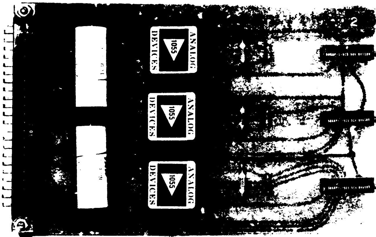
Figure 39. Board for Extra Operational Amplifiers (component side)
