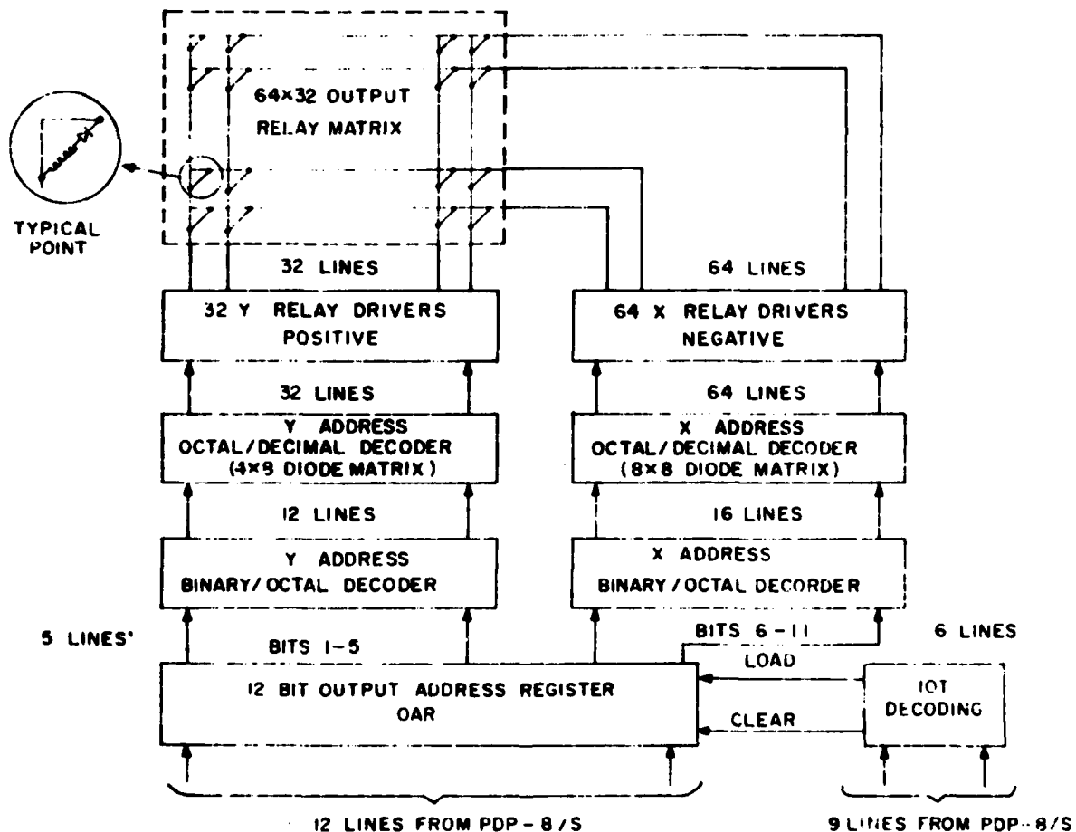
Figure 5. Block Diagram of the Controller Output Multiplexer
