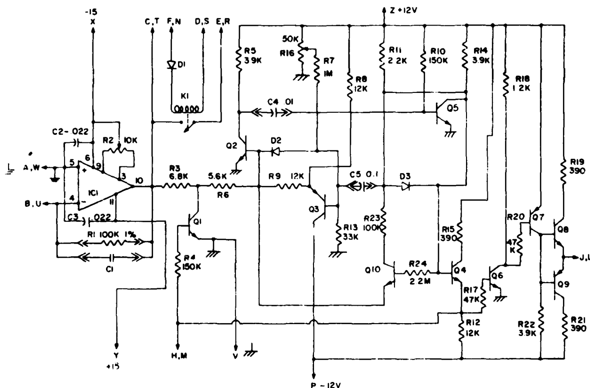
Figure 22. Mod 3 Sincoder Circuit
