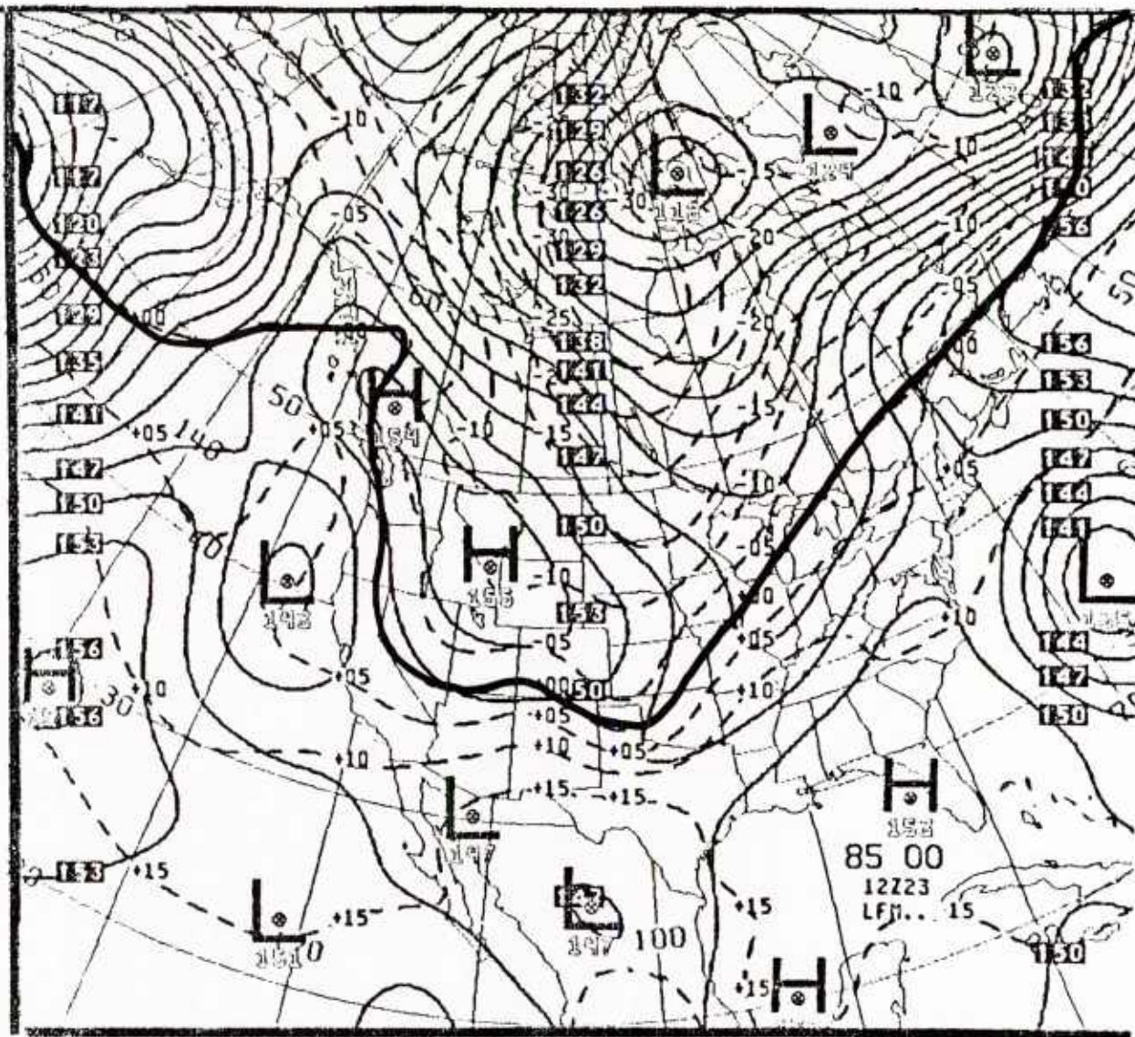
Figure 3. LFM 850-mb height and temperature analysis.
