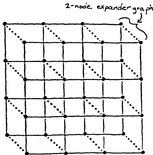
Figure 10. The expander-connected mesh P_{2,4} .
