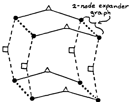
Figure 12. The expander-connected mesh of trees Q_{2,2} .
