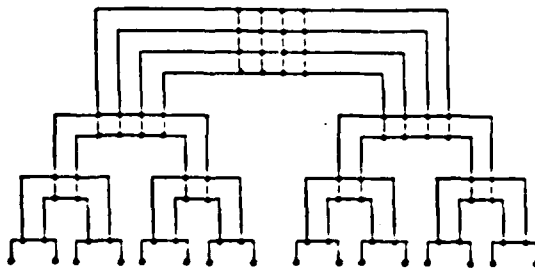
Figure 5. The 4 \times 4 tree of meshes T_4 .
