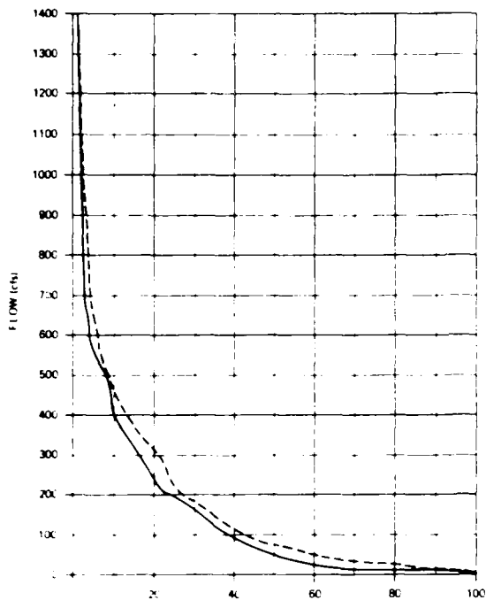
Des Plaines River at Gurnee 1 Day Flow Duration Simulated Vs. Recorded
