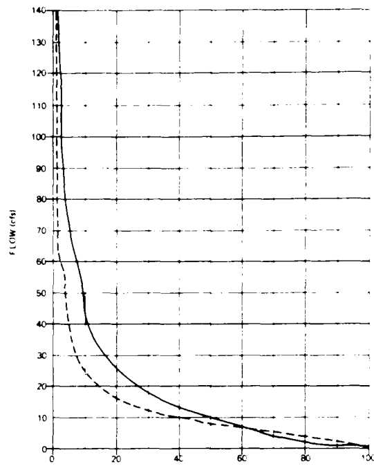
Buffalo Creek 1 Day Flow Duration Simulated Vs. Recorded
