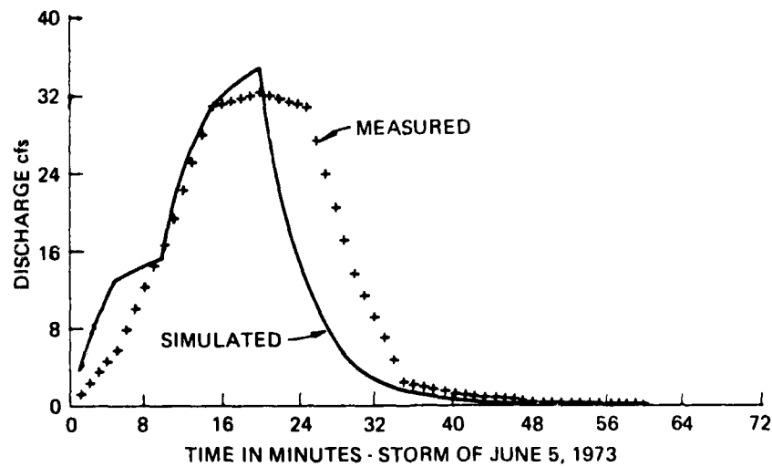
FIGURE 8 CLAIRMONT WATERSHED CALIBRATION RESULTS
