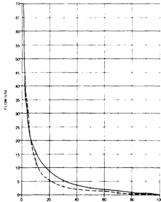
McDonald Creek 1 Day Flow Duration Simulated Vs. Recorded
