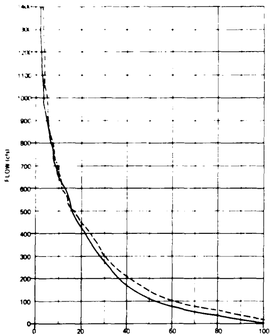
Des Plaines River Near Des Plaines 1 Day Flow Duration Simulated Vs. Recorded
