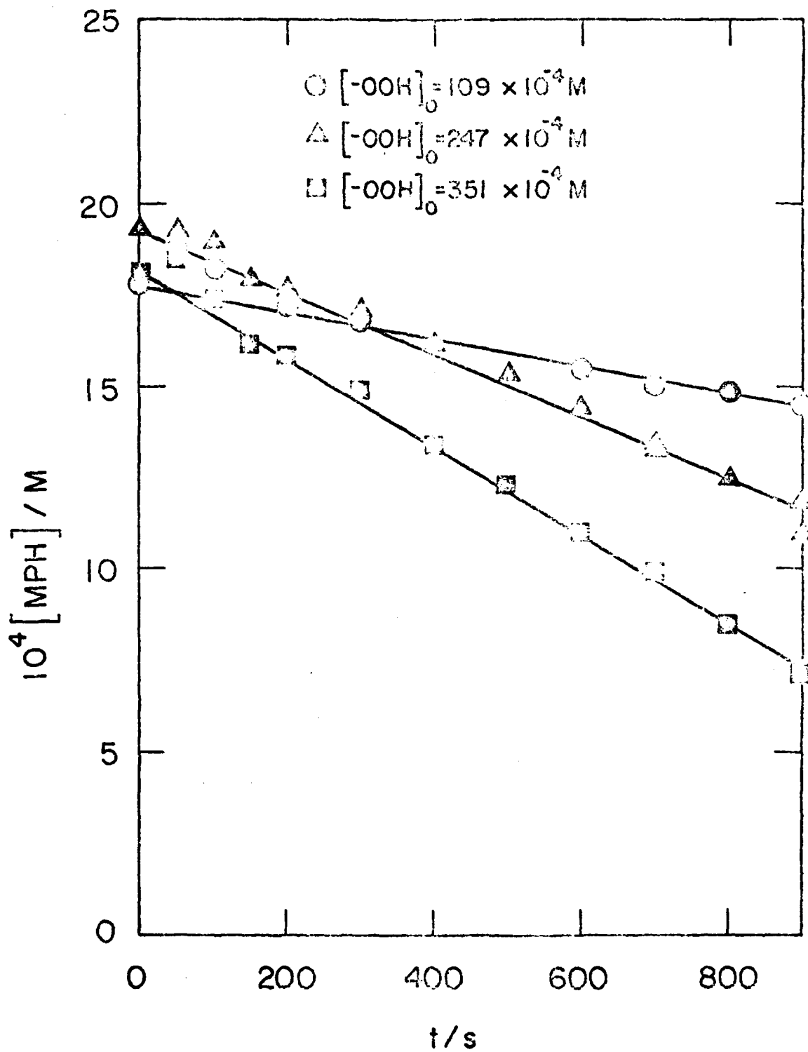
Figure 1. MPH decay during inhibited autoxidation of preoxidized H9 at 160°C.
