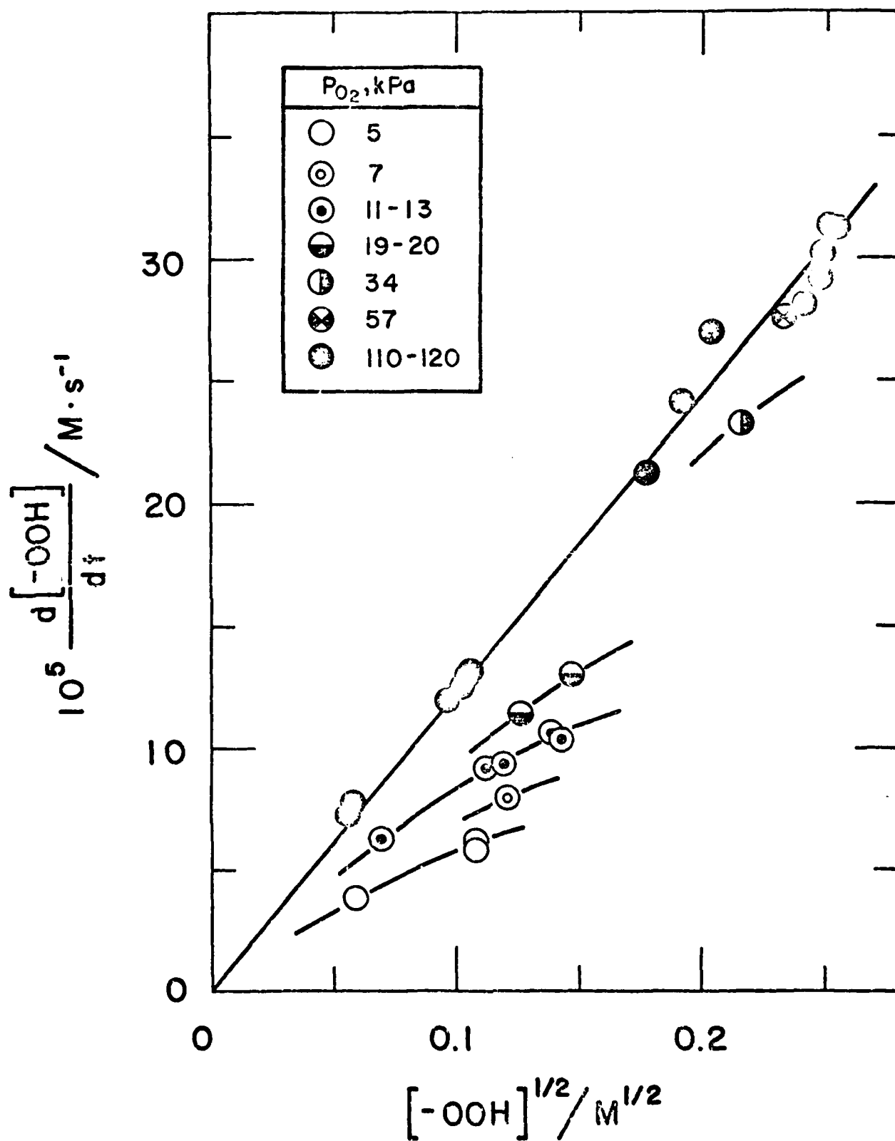
Figure 5 Rate of formation of hydroperoxides vs. [-OOH]^{1/2} at 180°C and at different oxygen pressures.
