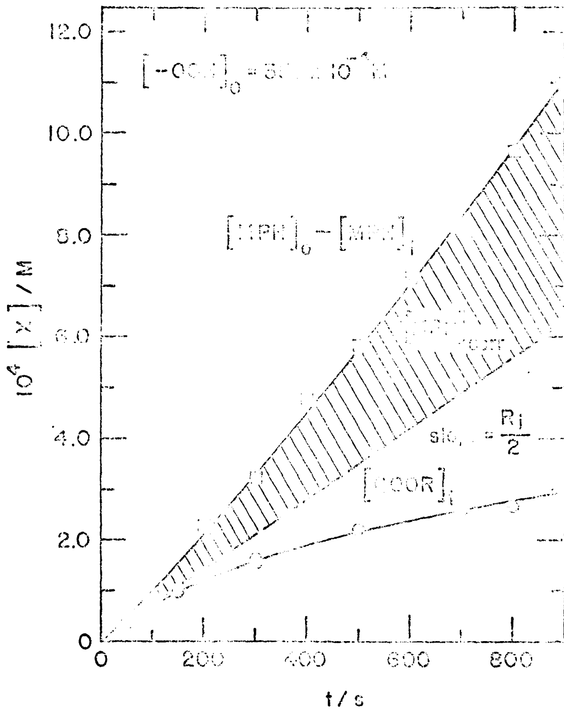
Figure 14 Consumption of MPH shown in Figure 3 corrected for MPH decay due to radical decomposition of COOR.
