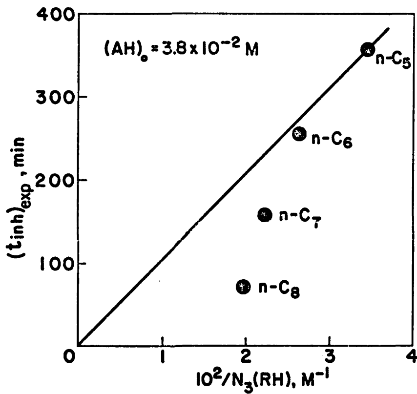
Figure 1. A plot of inhibition periods from the PAN inhibited autoxidation of straight-chain pentaerythrityl alkanooates at 232°C (1) vs. a reactivity parameter, 1/N_3(RH) .
