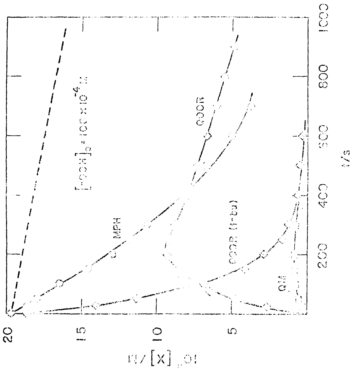
Figure 9. Addition of QOOR(1-bu) to MPH inhibited autoxidation of preoxidized QOOR (concentration of QOOR from 100).
