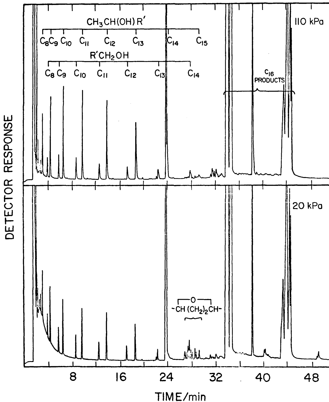
Figure 2 Chromatograms of oxy fractions from \text{NaBH}_4 reduced n -hexadecane oxidates ( 180^\circ\text{C} , runs 151 and 260) obtained using a bonded phase fused silica capillary column.
