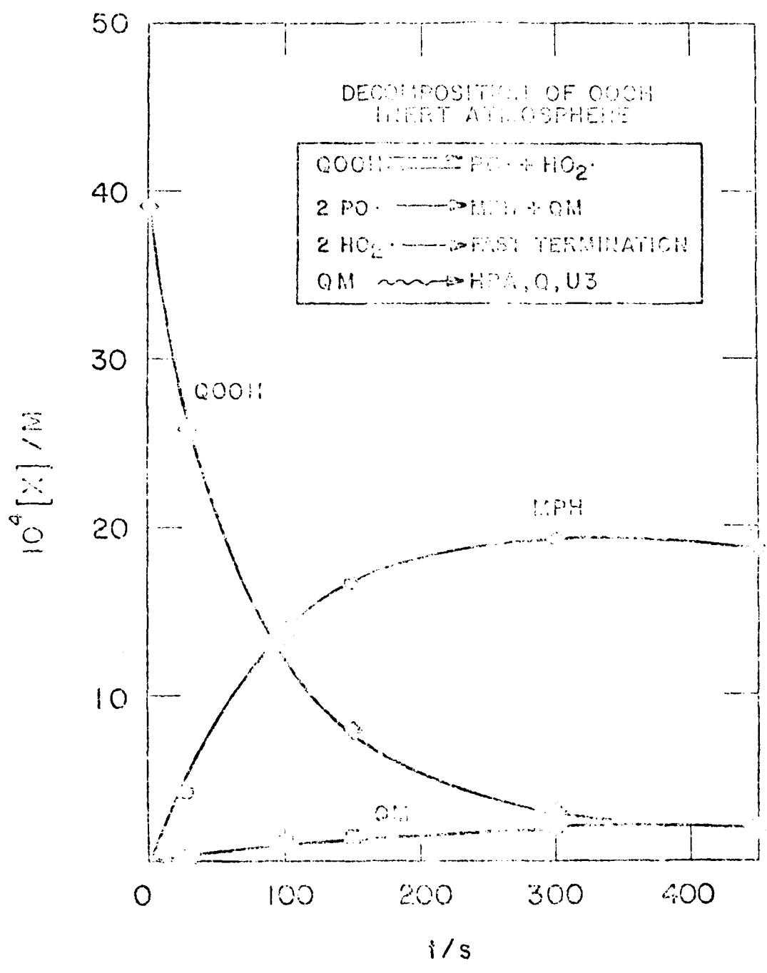
Figure 7 Thermal decomposition of QOOH under an inert atmosphere (Run 161).
