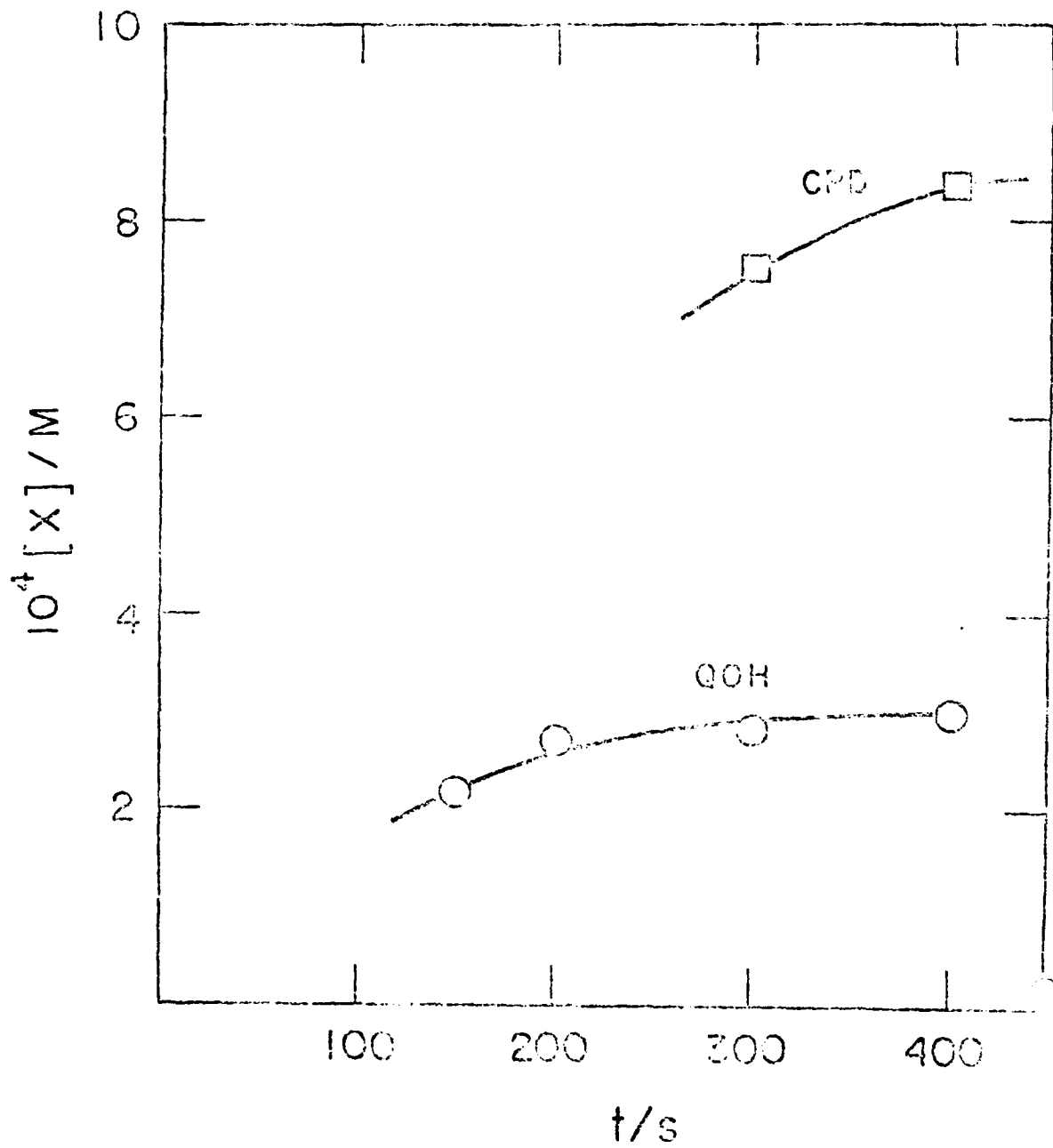
Figure 15. Formation of QOH and CPD upon addition of QOH into preoxidized II) at 120°C (run 105).
