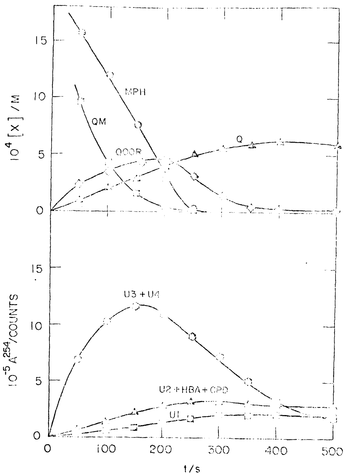
Figure 6 Decay of MPH and formation of products resulting from addition of 10^{-5} mole of into preoxidized n -hexane at 10^5 (run 150).
