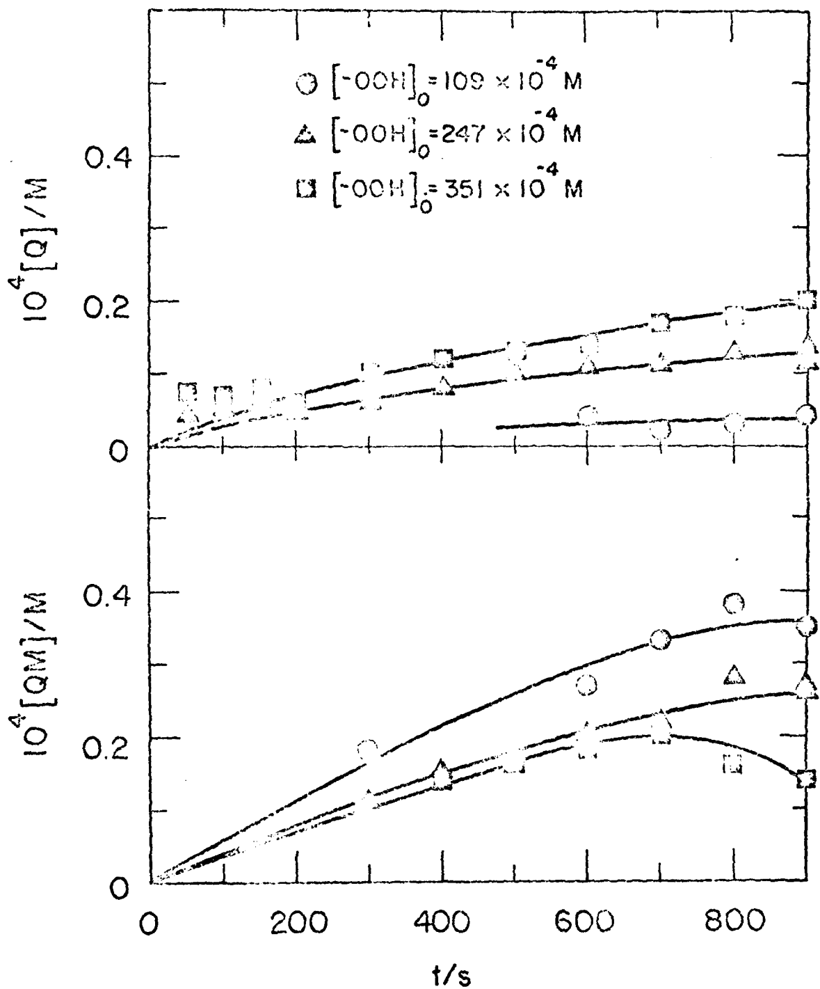
Figure 3. Formation of Q and QM during MPH inhibited autoxidation of preoxidized HD at 160°C.
