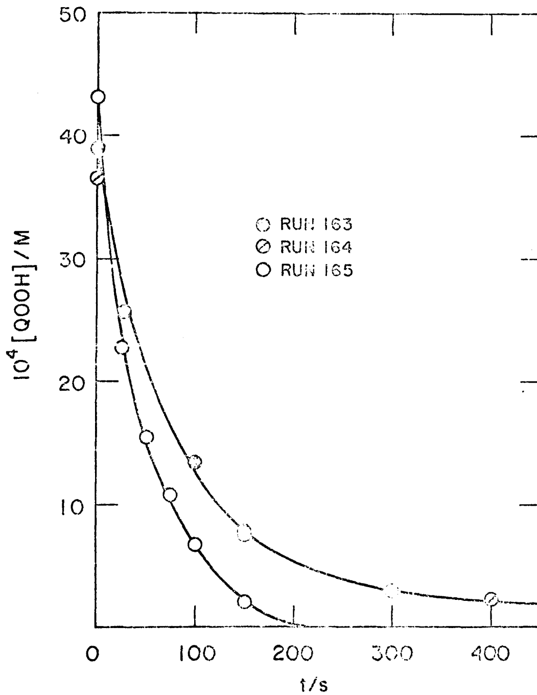
Figure 11. Decay of QOOH upon addition into HD at 180^\circ\text{C} .
