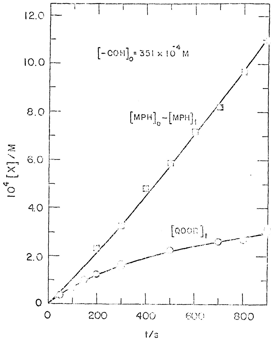
Figure 3 Formation of QOR and consumption of MPH during MPH inhibited autoxidation of preoxidized n -hexadecane at 100°C.
