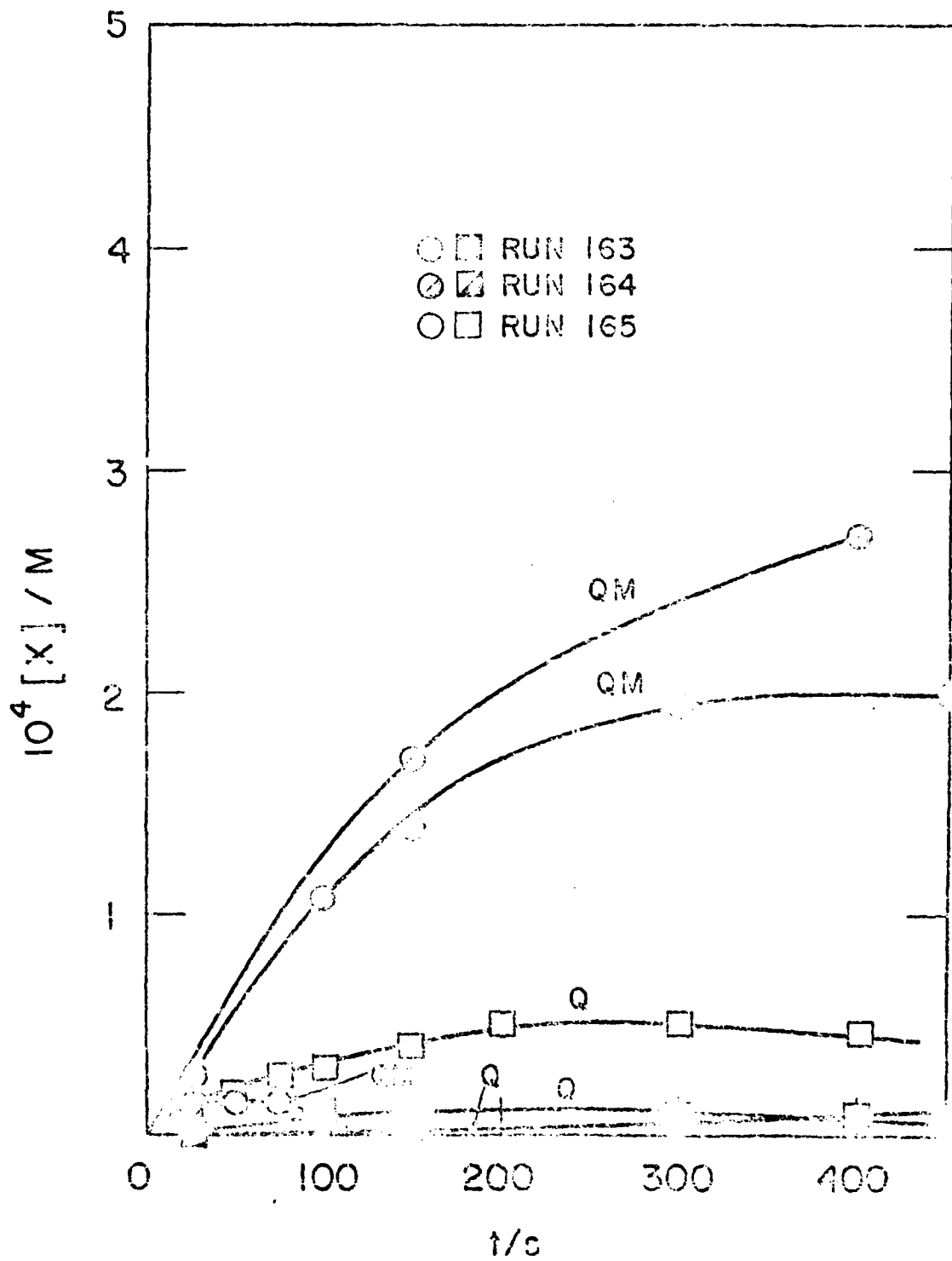
Figure 13. Formation of QM and Q upon addition of QOH into HD at 180°C.
