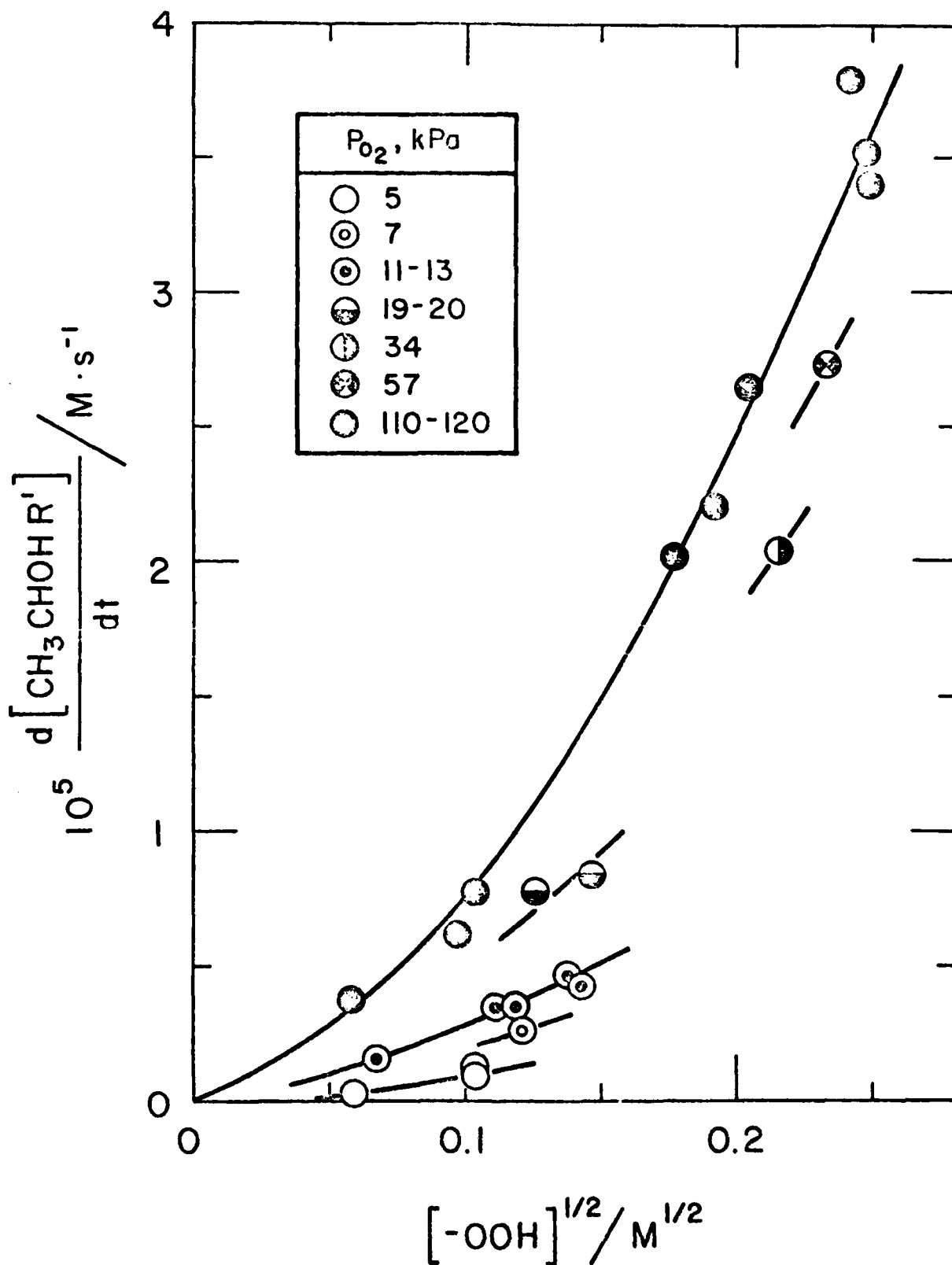
Figure 12 Rate of formation of cleavage methyl ketones vs. [-OOH]^{1/2} at 180°C and different oxygen pressures.
