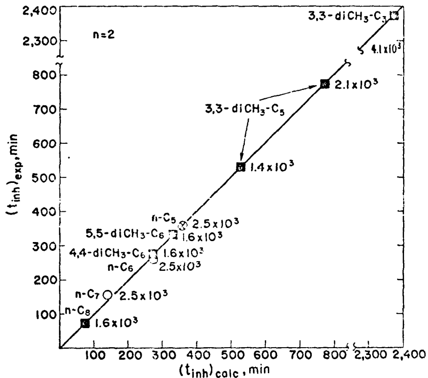
Figure 4. A plot of experimental values of t_{inh} versus calculated values of t_{inh} for various hydrocarbons. The calculated values are the values of t_{inh} calculated from the rate constants of the reaction of the hydrocarbons with SO_2 dissolved in the liquid.
