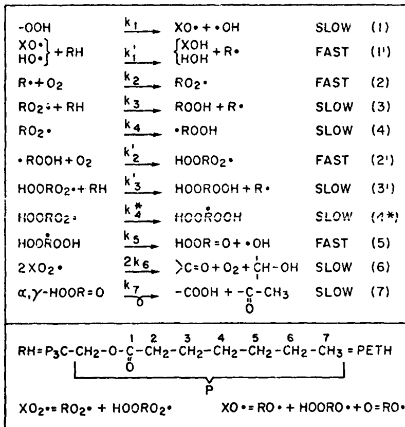
Fig. 12. Reaction scheme for the autoxidation of PETH.
