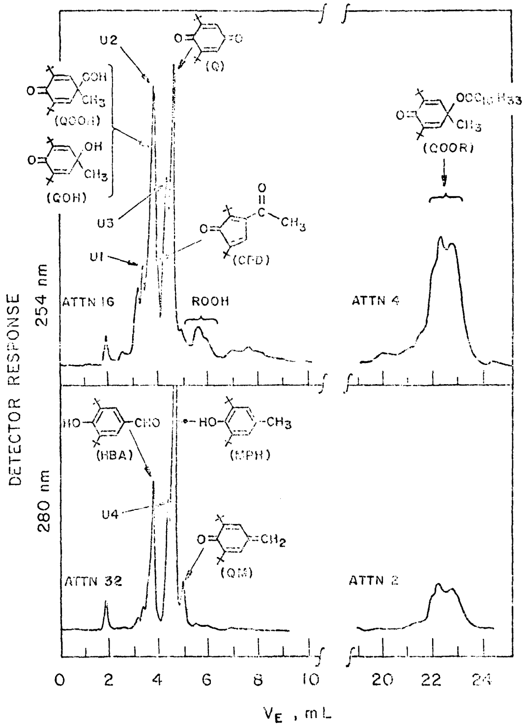
Figure 4. HPLC separation of sample from HPL inhibited autooxidation of peroxidized n -hexadecane at 150°C.
