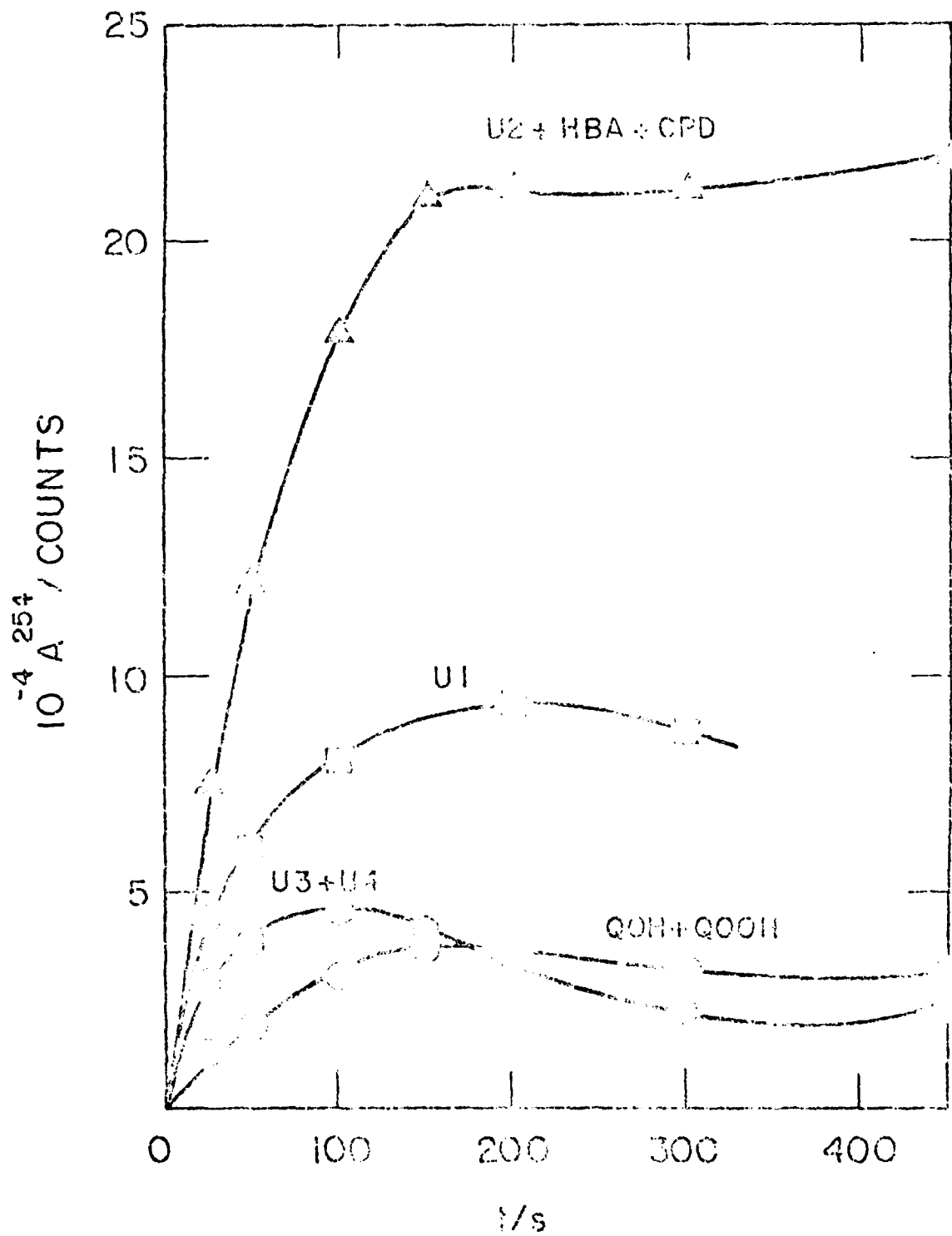
Figure 17. Product formation upon addition of q\text{O}^{\bullet}(\text{tBu}) into preoxidized HD at 150^{\circ}\text{C} (run 161).
