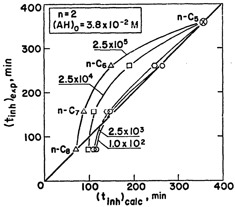
Figure 3. Plots of experimental inhibition periods from the PAN inhibited autoxidation of straight-chain pentaerythrityl alkanoses at 232°C (1) vs. corresponding values calculated from Eq. VIII as a function of k_6/(k_3/H) .
