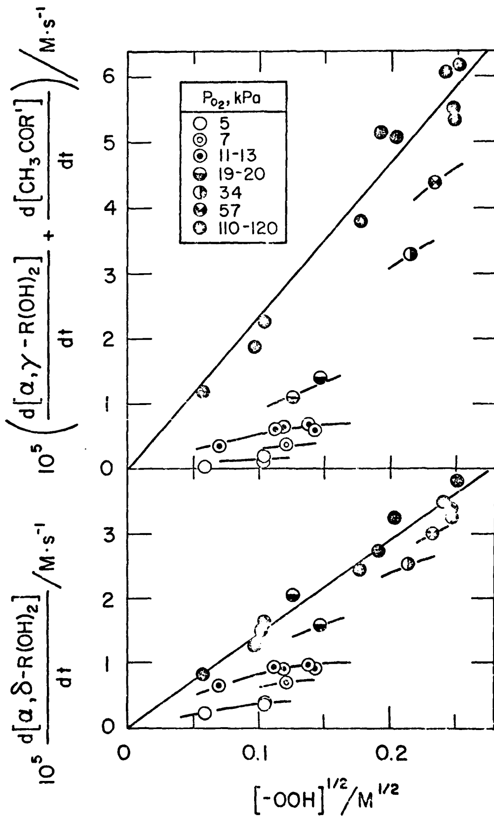
Figure 6 Rates of formation of difunctional products vs. [-OOH]^{1/2} at 180°C and at different oxygen pressures.
