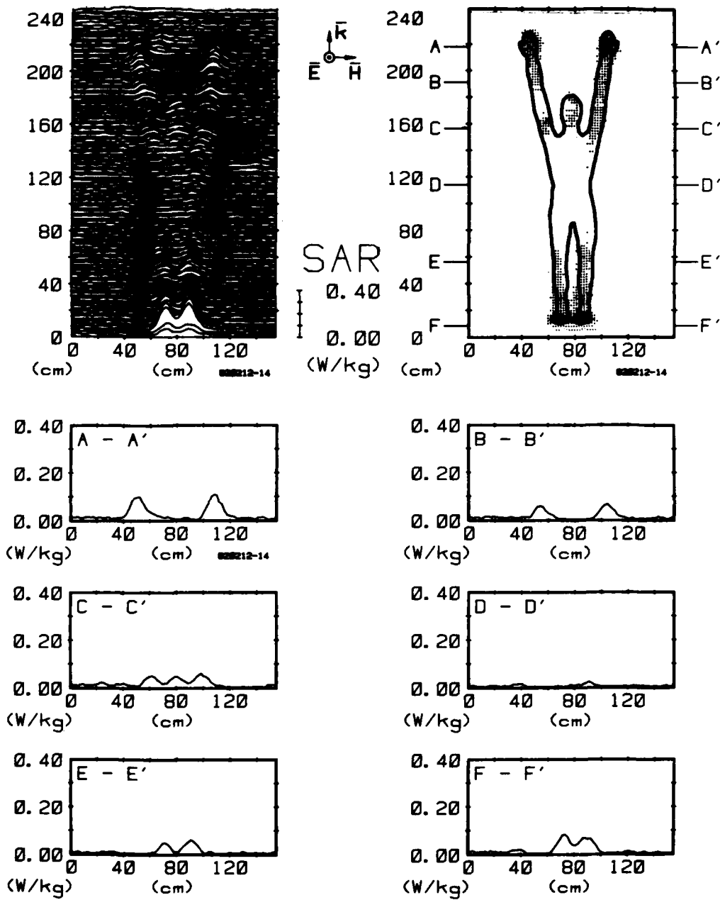
Figure 40. Computer-processed whole-body thermograms expressing SAR patterns for man with arms up, exposed to 1\text{-mW/cm}^2 450-MHz radiation with KHE polarization.
