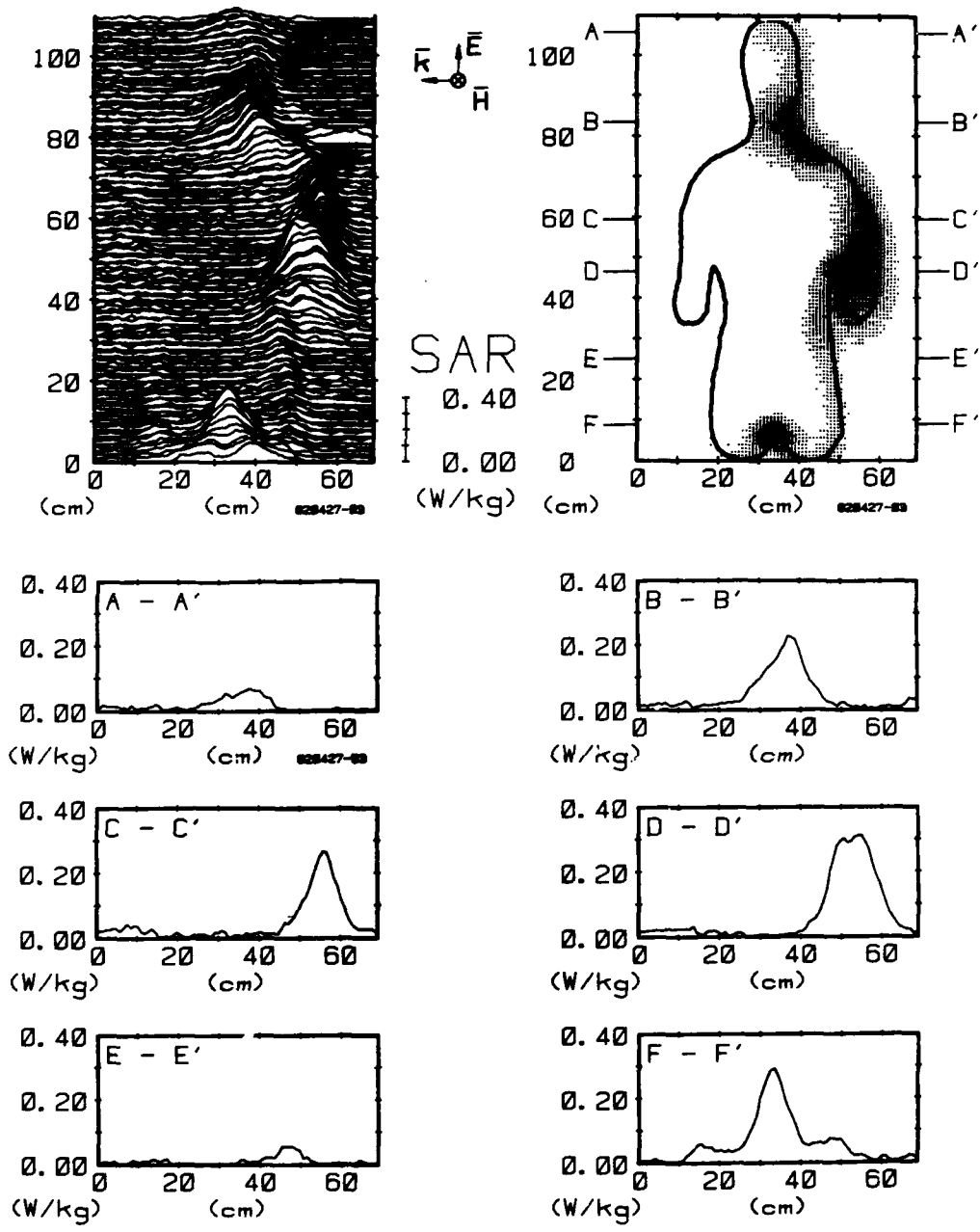
Figure 59. Computer-processed whole-body thermograms expressing SAR patterns for man sitting (frontal plane), exposed to 1-mW/cm 2 450-MHz radiation with EKH polarization.
