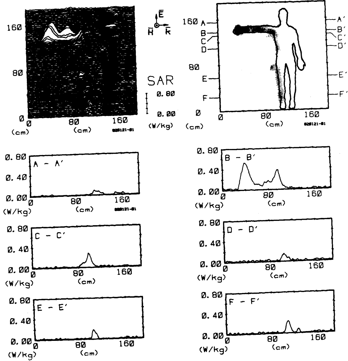
Figure 45. Computer-processed whole-body thermograms expressing SAR 2 patterns for man with one arm extended, exposed to 1-mW/cm 2 450-MHz radiation with -EKH polarization.
