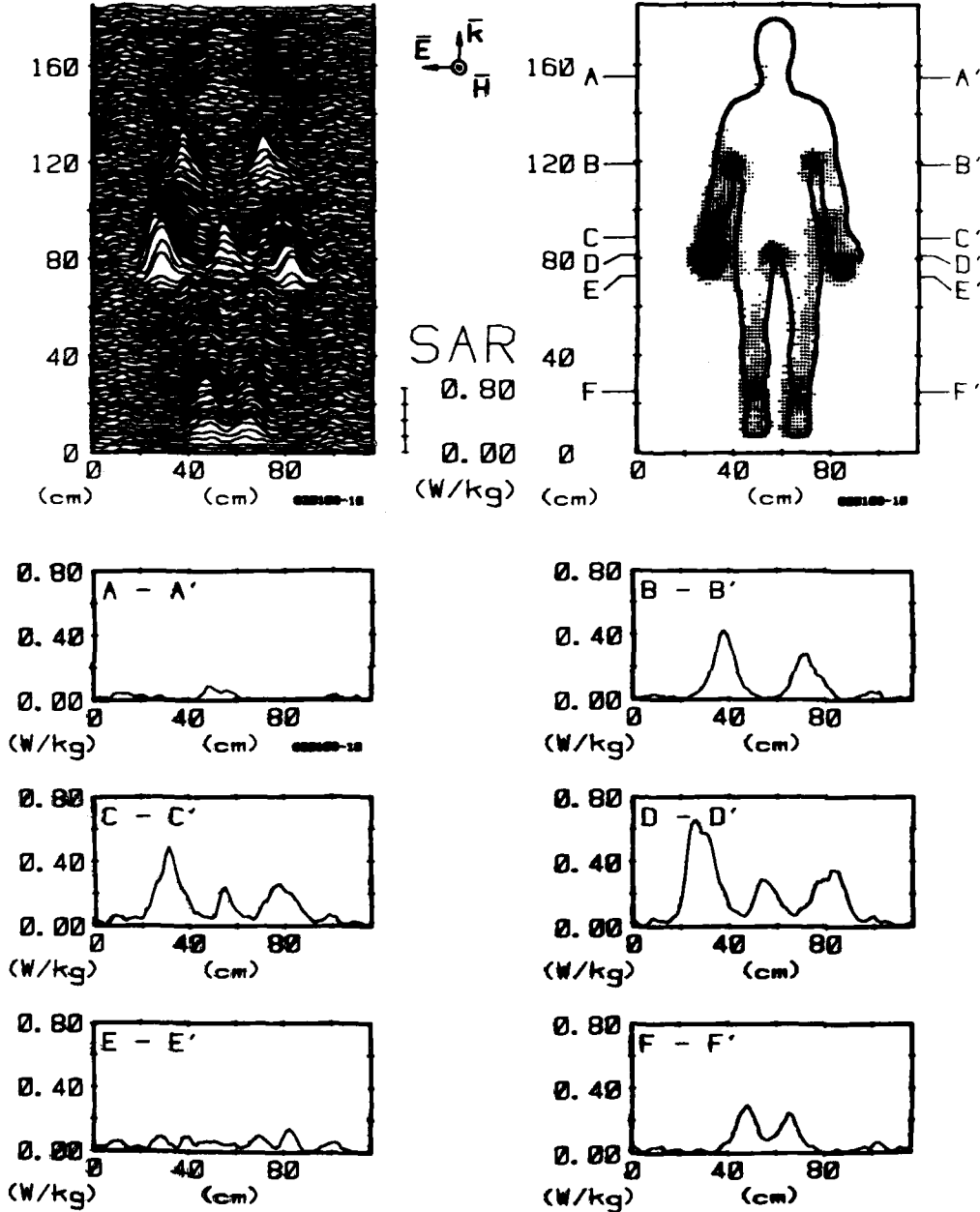
Figure 28. Computer-processed whole-body thermograms expressing SAR patterns for man with arms down, exposed to 1\text{-mW/cm}^2 450-MHz radiation with KEH polarization.
