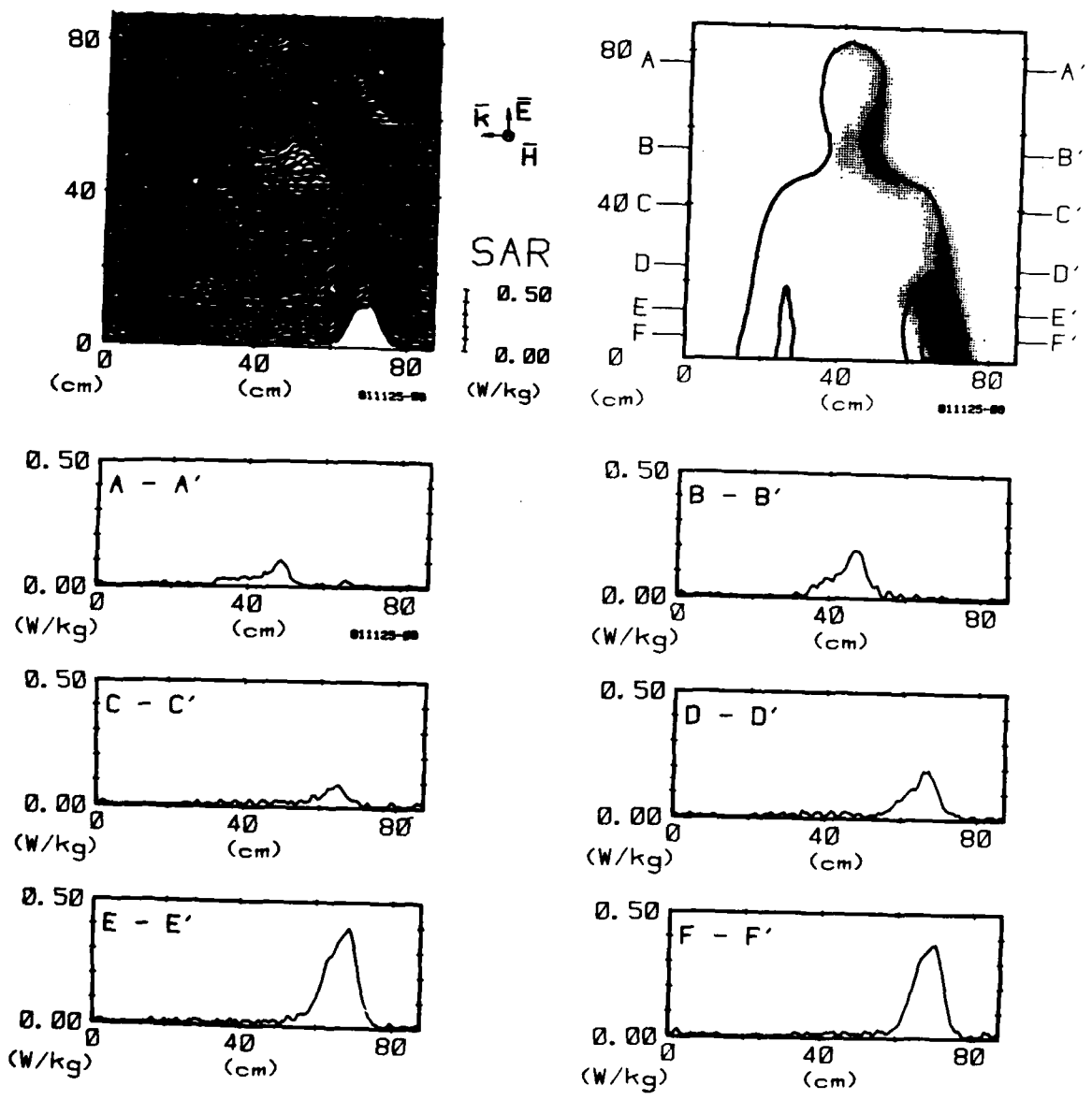
Figure 24B. Computer-processed upper-body thermograms expressing SAR patterns for man with arms down, exposed to 1-mW/cm 2 450-MHz radiation with EKH polarization.
