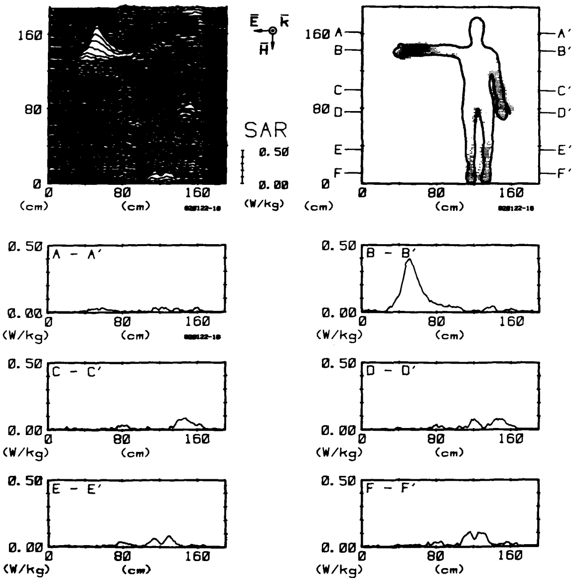
Figure 47. Computer-processed whole-body thermograms expressing SAR patterns for man with one arm extended, exposed to 1-mW/cm 2 450-MHz radiation with -HEK polarization.
