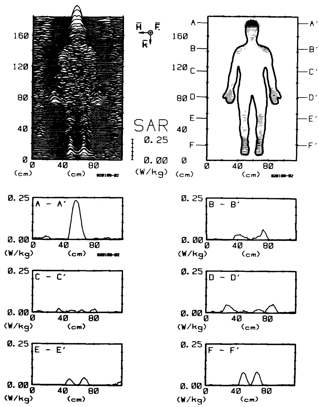
Figure 31. Computer-processed whole-body thermograms expressing SAR patterns for man with arms down, exposed to 1-mW/cm 2 450-MHz radiation with -KHE polarization.
