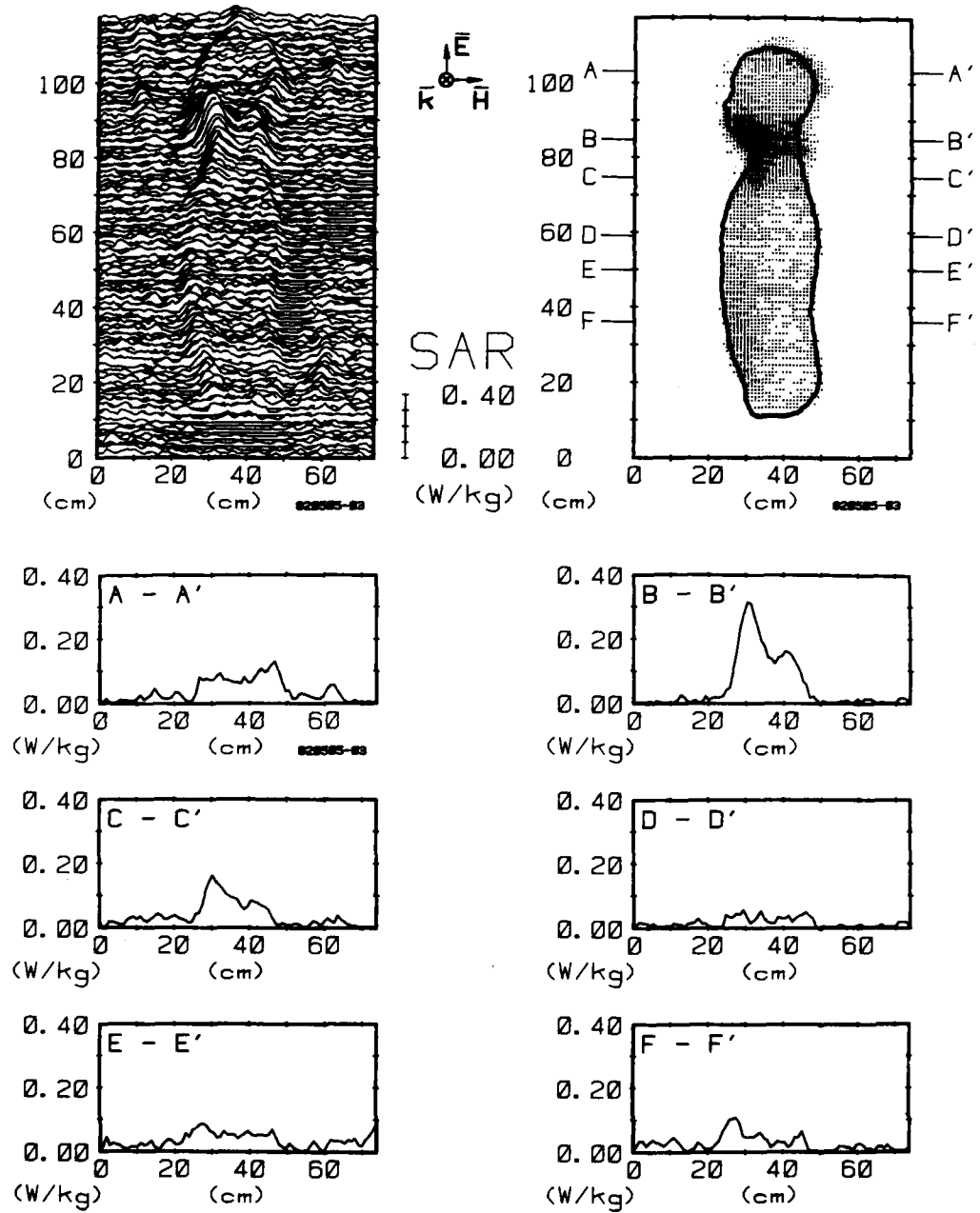
Figure 54. Computer-processed whole-body thermograms expressing SAR patterns for man sitting (sagittal plane), exposed to 1\text{-mW/cm}^2 450-MHz radiation with EHK polarization.
