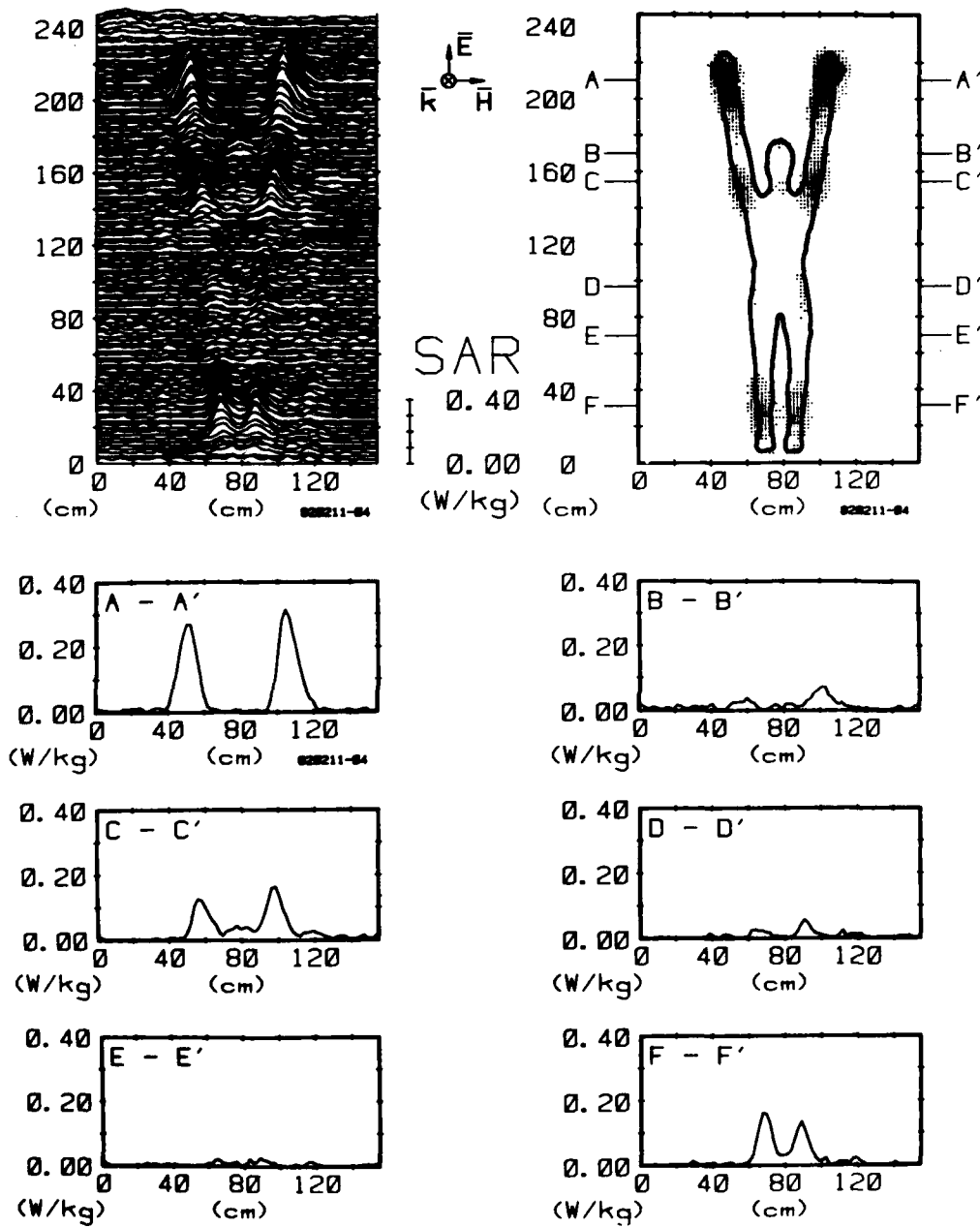
Figure 32. Computer-processed whole-body thermograms expressing SAR patterns for man with arms up, exposed to 1\text{-mW/cm}^2 450-MHz radiation with EHK polarization.
