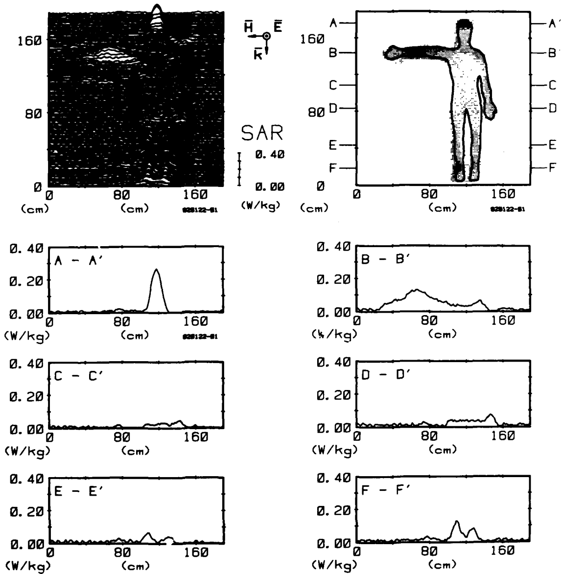
Figure 53. Computer-processed whole-body thermograms expressing SAR 2 patterns for man with one arm extended, exposed to 1-mW/cm 2 450-MHz radiation with -KHE polarization.
