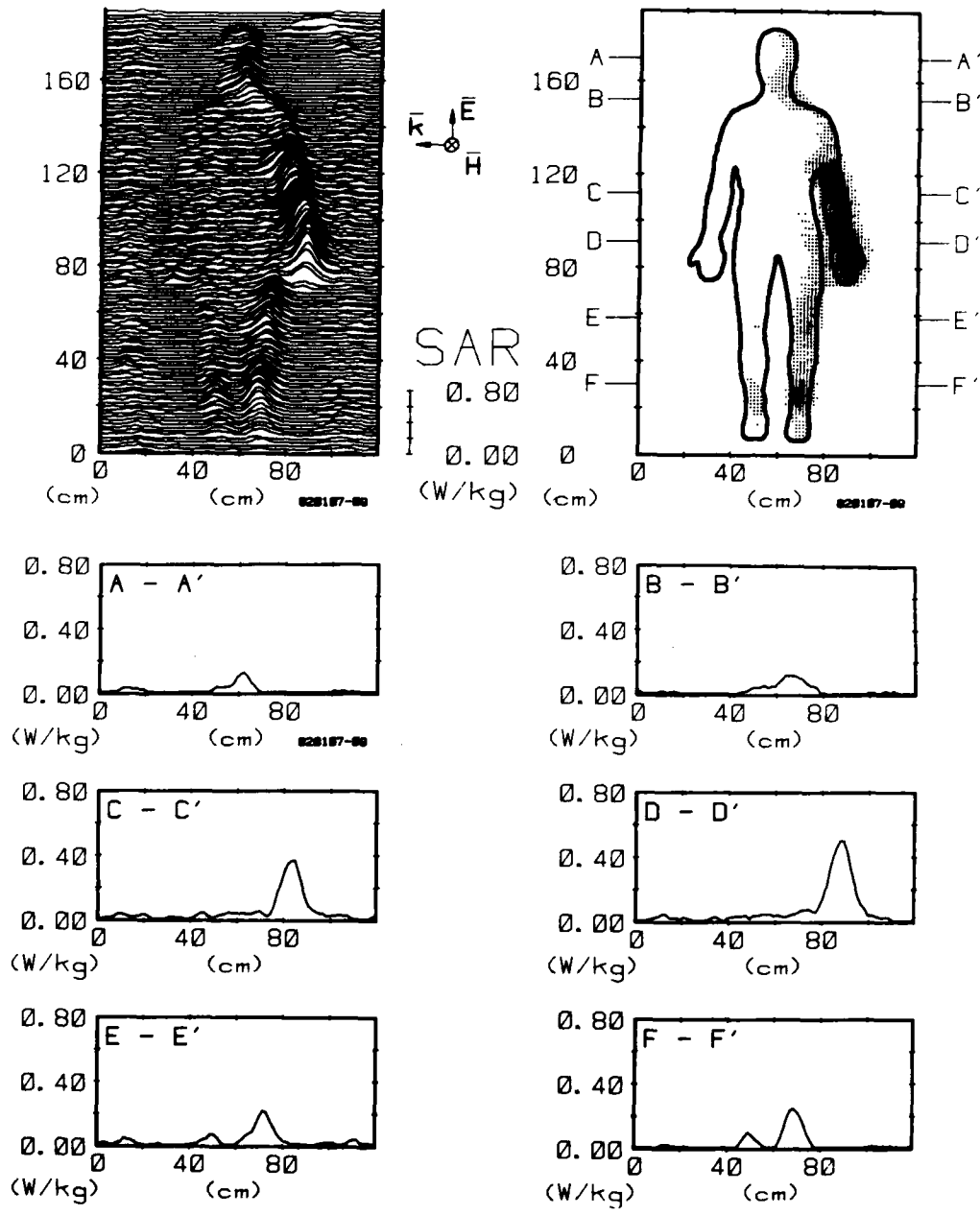
Figure 24A. Computer-processed whole-body thermograms expressing SAR patterns for man with arms down, exposed to 1\text{-mW/cm}^2 450-MHz radiation with EKH polarization.
