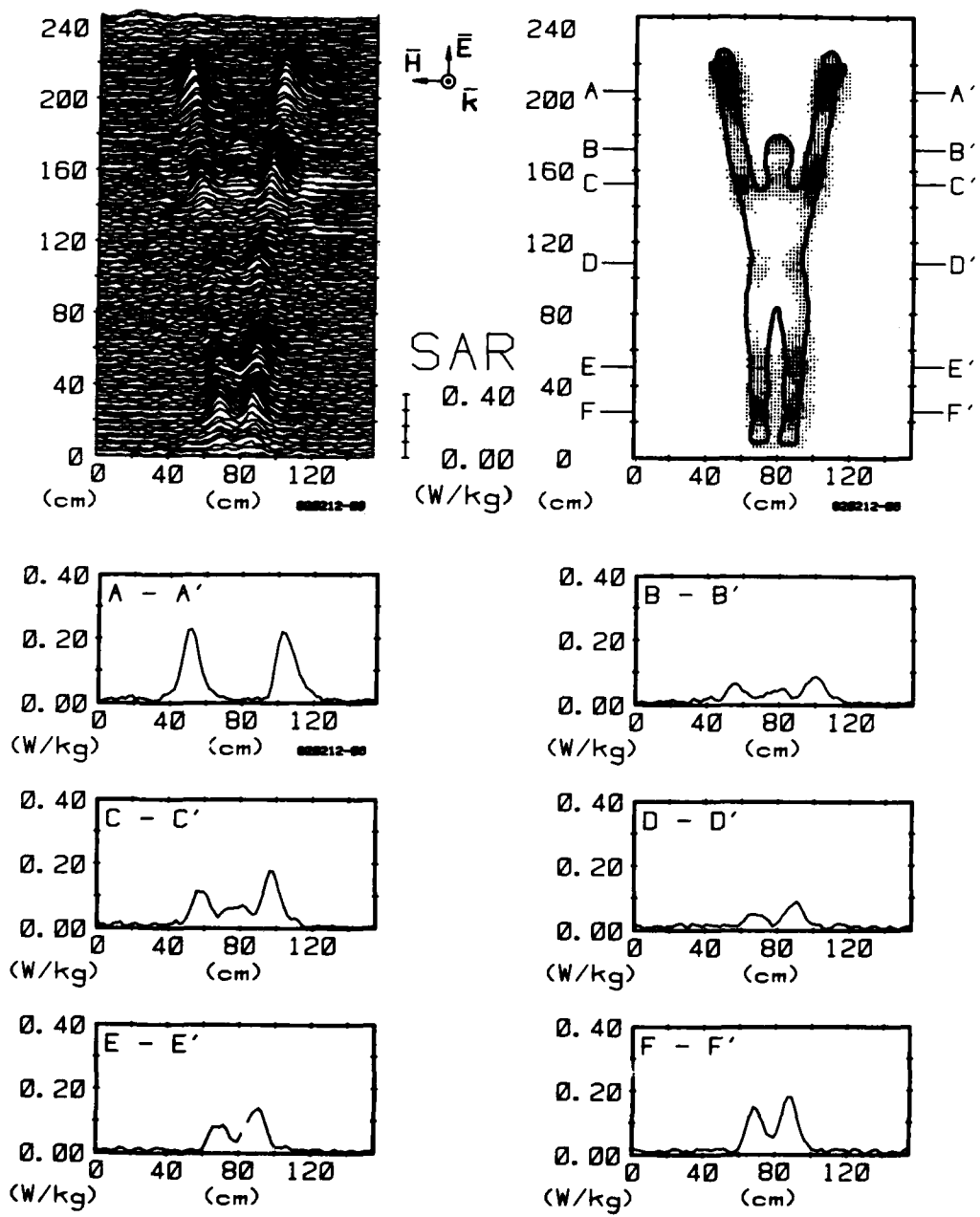
Figure 33. Computer-processed whole-body thermoqrms expressing SAR patterns for man with arms up, exposed to 1\text{-mW/cm}^2 450-MHz radiation with -EHK polarization.
