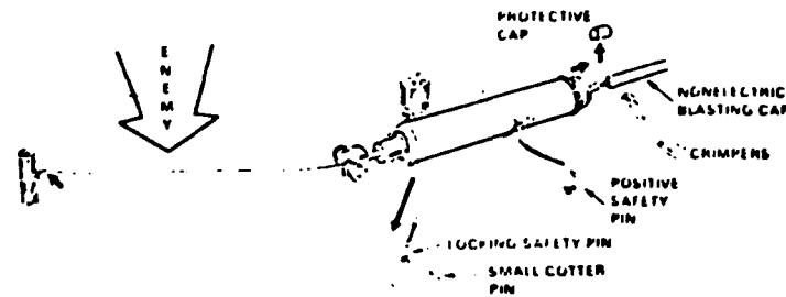
Figure 4-3. Product specification in a mechanical assembly (11C, p. 2-II-C-10.4)
