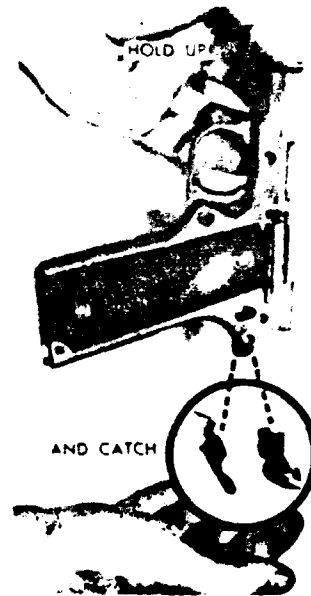
Figure 4(2). Disassembly of receiver group.
