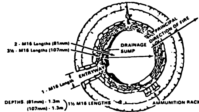
Figure 4-2. Specifying standards characteristics for a "construction" task (11C,* p. 2-II-B-10.1)
