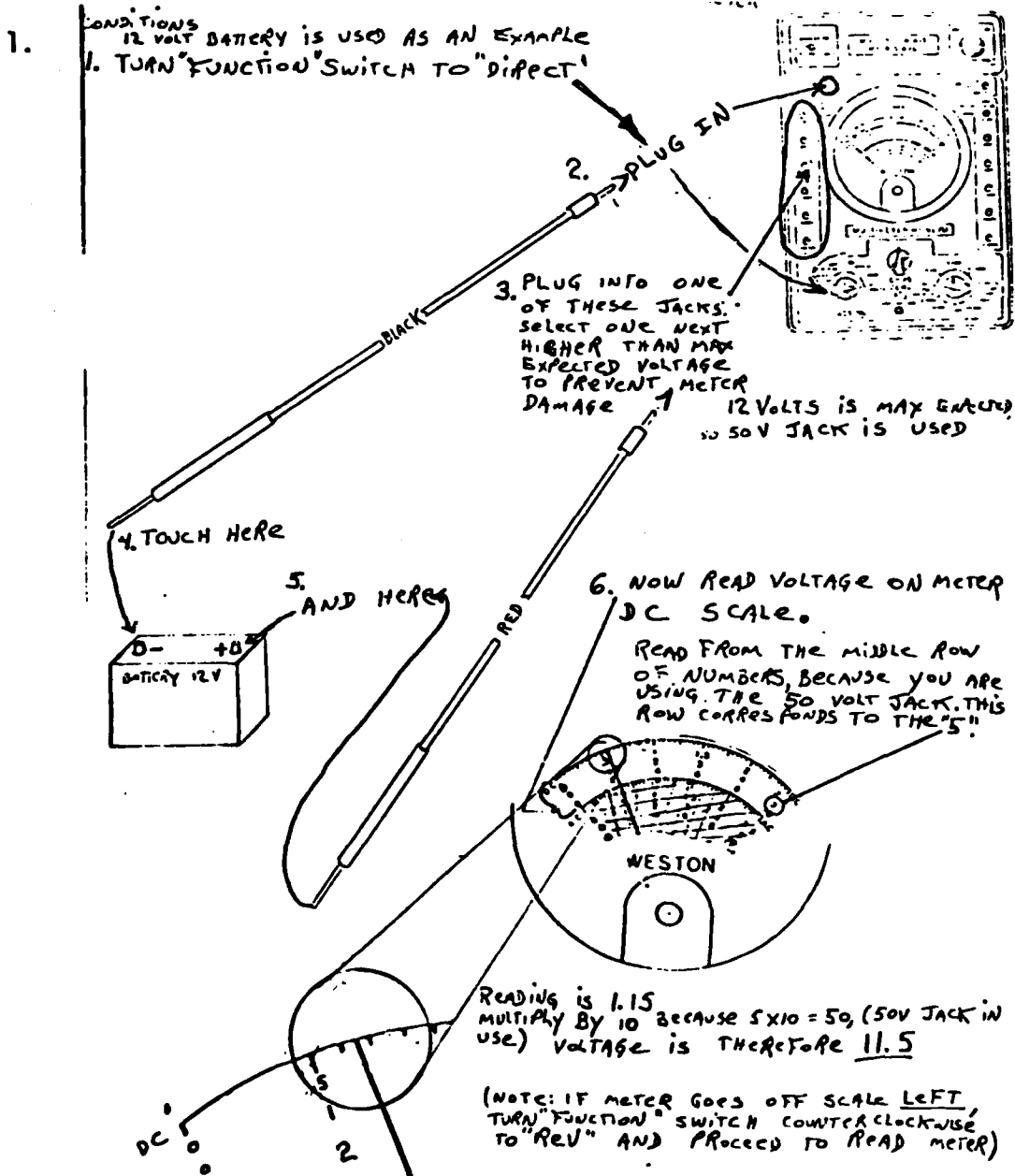
Figure 4-13. Measuring voltage, 12 volt battery.
