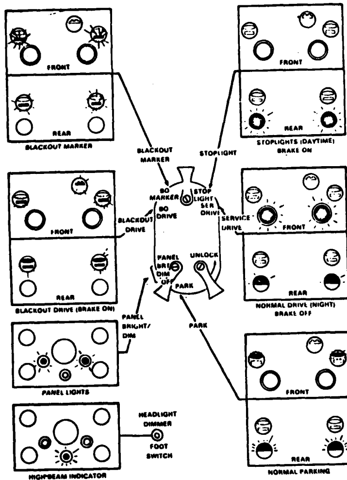
Figure 4-19. Signals, meaning (11C, p. 2-VII-A-3.3)
