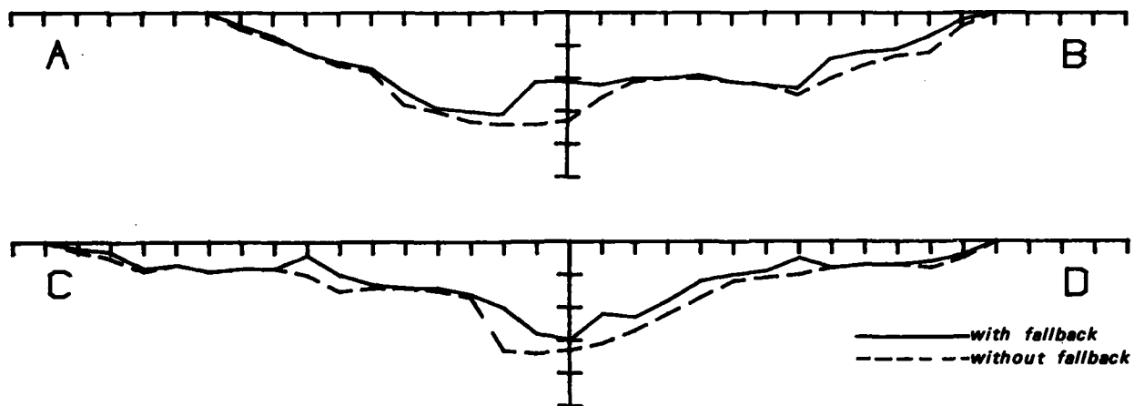
Figure D-11. Crater 4 (155mm--Mindi Farm) Profile Comparisons--with and without Fallback.
