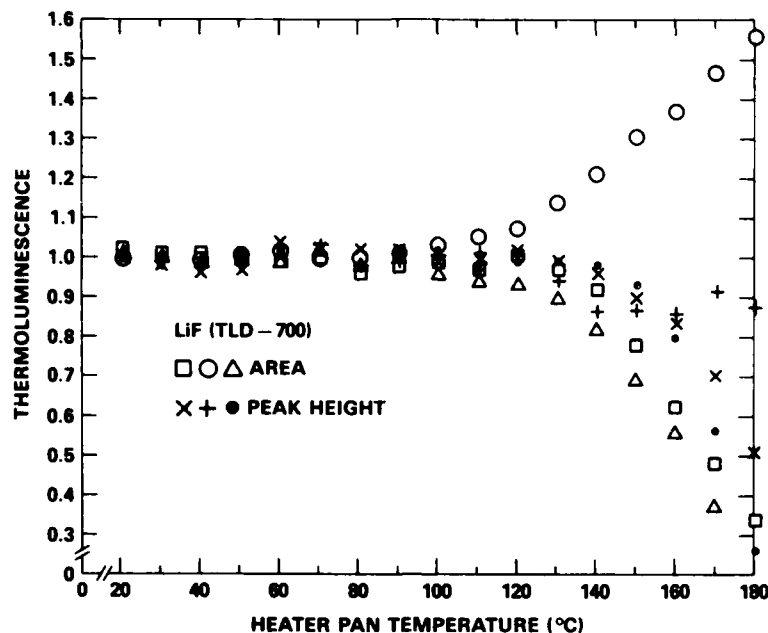
Fig. 4 — Response of LiF(TLD-700) thermoluminescence dosimeters vs annealing temperatures for: dosimeters annealed for 1 min after exposure at 22°C (□, ×); dosimeters annealed for 1 min prior to exposure at 22°C (○, ●); and dosimeters annealed for 30 s before and after exposure at 22°C (△, ●). All dosimeters were given a low-temperature anneal at 80°C for 16 h prior to the experiment.
