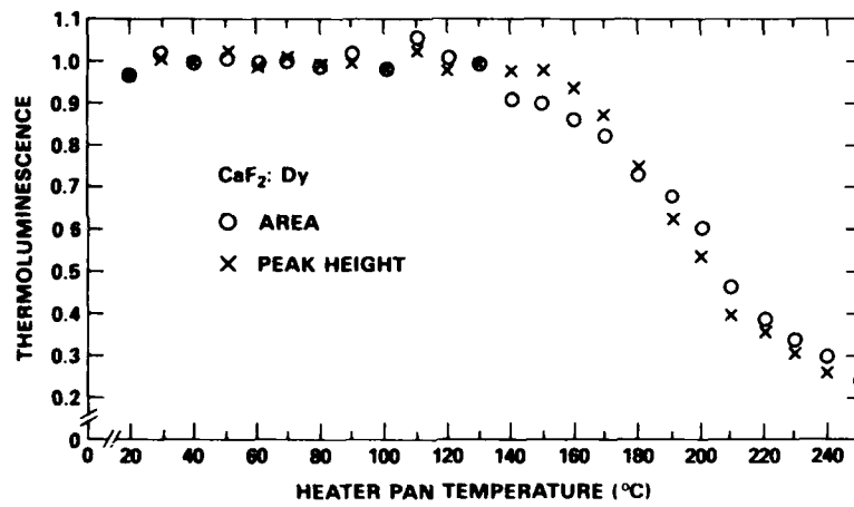
Fig 6 — Response of CaF 2 :Dy thermoluminescence dosimeters as a function of temperature during irradiation
