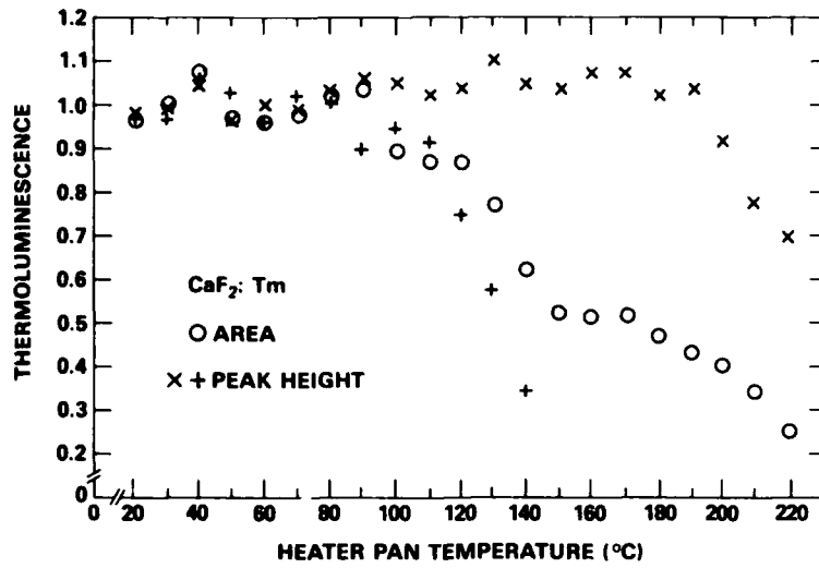
Fig. 7 — Response of \text{CaF}_2:\text{Tm} thermoluminescence dosimeters as a function of temperature during irradiation (+, 150^\circ\text{C} peak height; x, 240^\circ\text{C} peak height)
