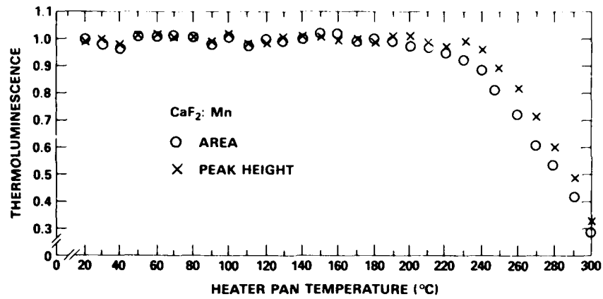
Fig. 5 — Response of CaF 2 :Mn thermoluminescence dosimeters as a function of heater pan temperature during irradiation
