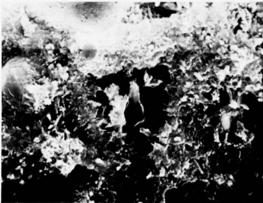
Figure 2. Micrograph 072380-15, X 5300. Fracture surface of Mixture M-8-B at 7-day age. Normal hydration products and residual cement grains.
