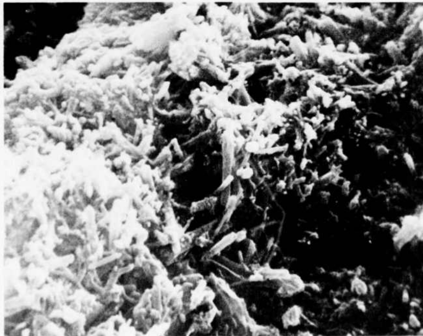
Figure 5. Micrograph 080680-26, X 5000. Fracture surface of Mixture M-8-E at 7-day age. Enlargement of part of Figure 18 shows ettringite crystals in void, calcium hydroxide (upper center), CSH, and void space.
