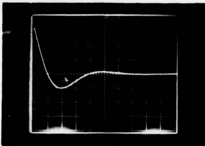
FIGURE A-14. 2-POLE 1 DB-RIPPLE CHEBYSHEV HIGH-PASS RESPONSE
