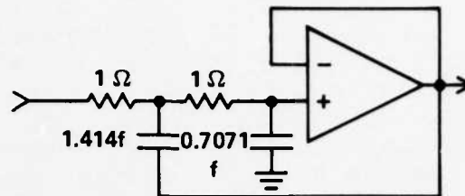
A. NORMALIZED LOW-PASS FILTER
