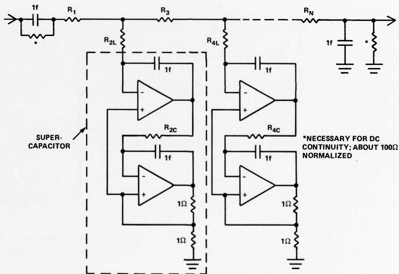
B. ACTIVE LOW-PASS
