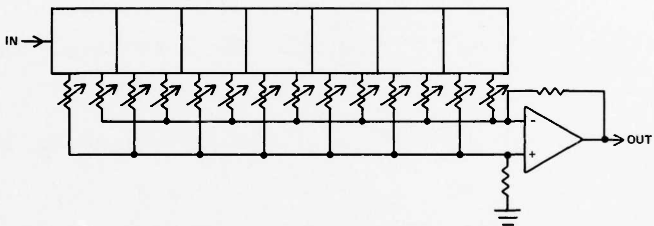
FIGURE 27. TRANSVERSAL FILTER
