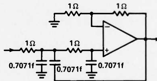
c. LOW-PASS, GAIN OF 2
