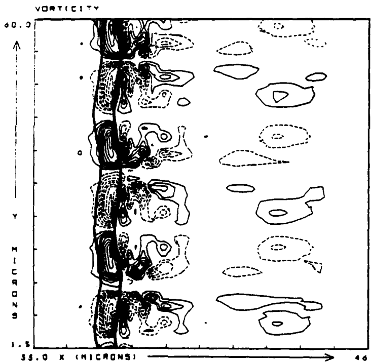
Figure 6. Vorticity contours for the 20 \mu\text{m} mode ( \lambda/\Delta R = 1 ) when the system is in the linear regime. The contours are in 10% increments of the maximum vorticity ( +2.75 \times 10^8 , -2.87 \times 10^8 \text{ S}^{-1} ). The solid (dashed) contours are positive (negative) vorticity. The heavy lines delineate the 10% (right) and 90% (left) density contour.
