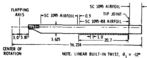
Figure 4.- Rotor blade geometry. Blade dimensions are in inches.
