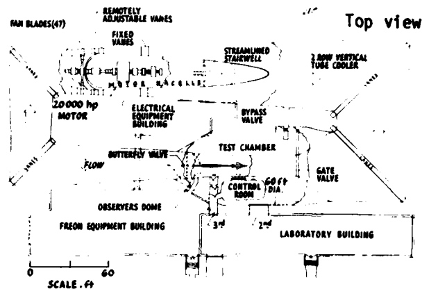
Figure 1.- Langley Transonic Dynamics Tunnel.
