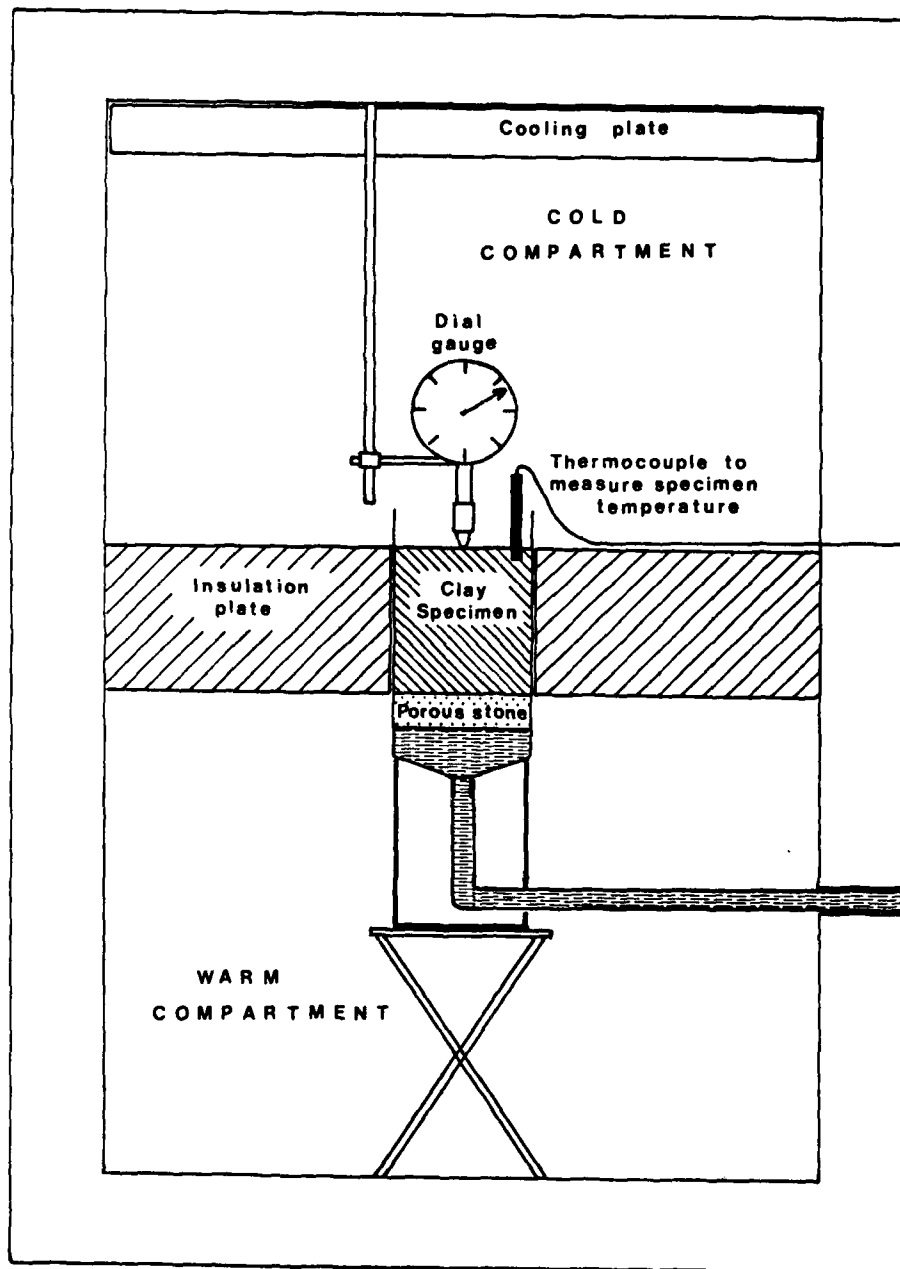
Fig. 1: System sketch of freezer for clay testing with cold compartment in the upper part and warm compartment in the lower part for steady water flow into the sample
