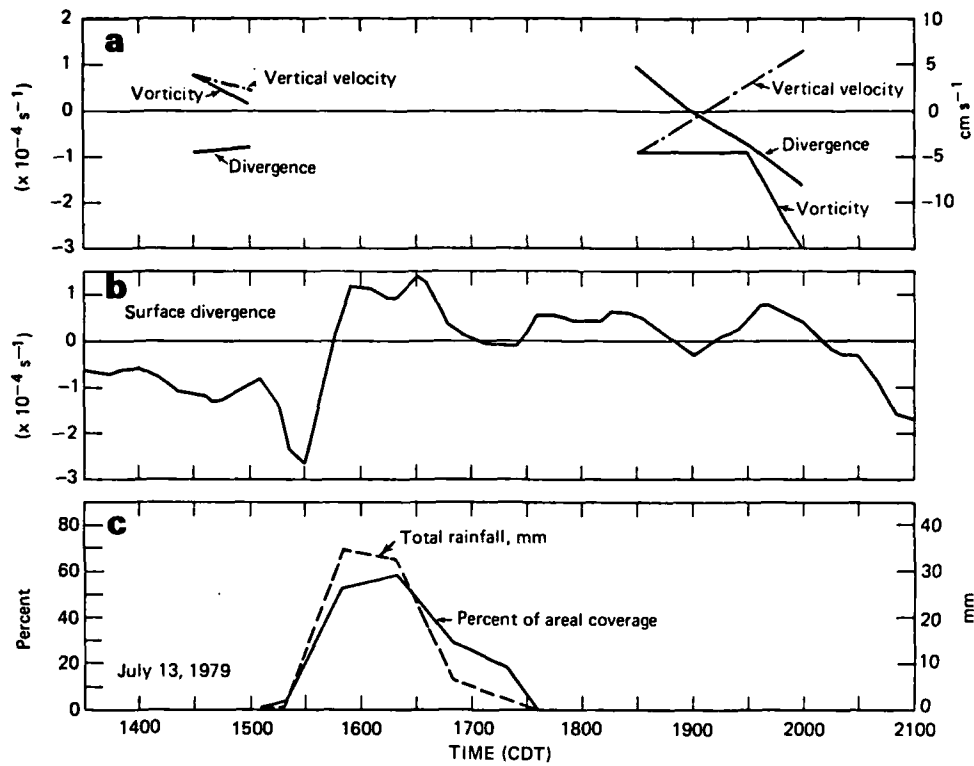
Figure 3. Time series of (a) column-average (300-700 m MSL) divergence and vorticity ( 10^{-4} s^{-1} ) and vertical motion at 700 m MSL ( cm s^{-1} ), (b) surface divergence and (c) total 30-min rainfall and percent of area covered, all for pibal triangle, on 13 July 1979.
