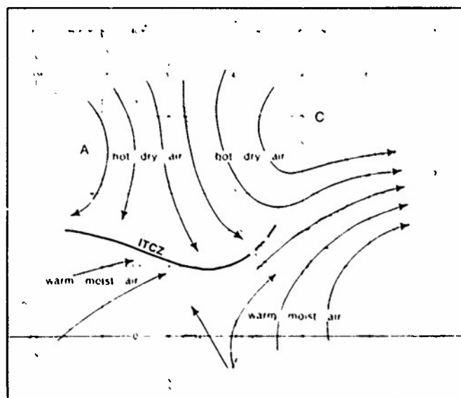
11-1b Typical summer air mass movement over Red Sea-Persian Gulf
