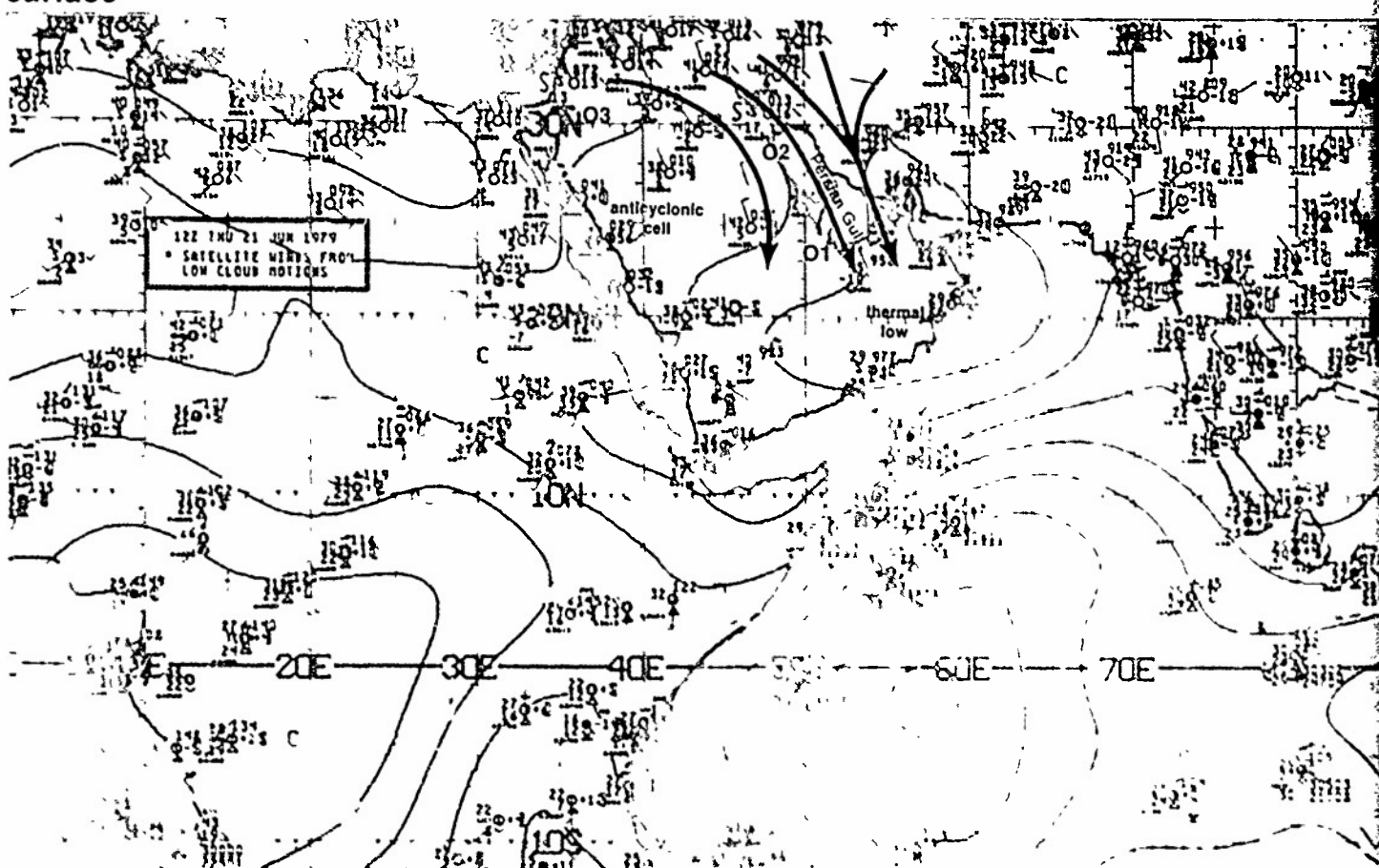
1E-20b NMC Tropical Surface Streamline Analysis 1200 GMT 21 June 1979
