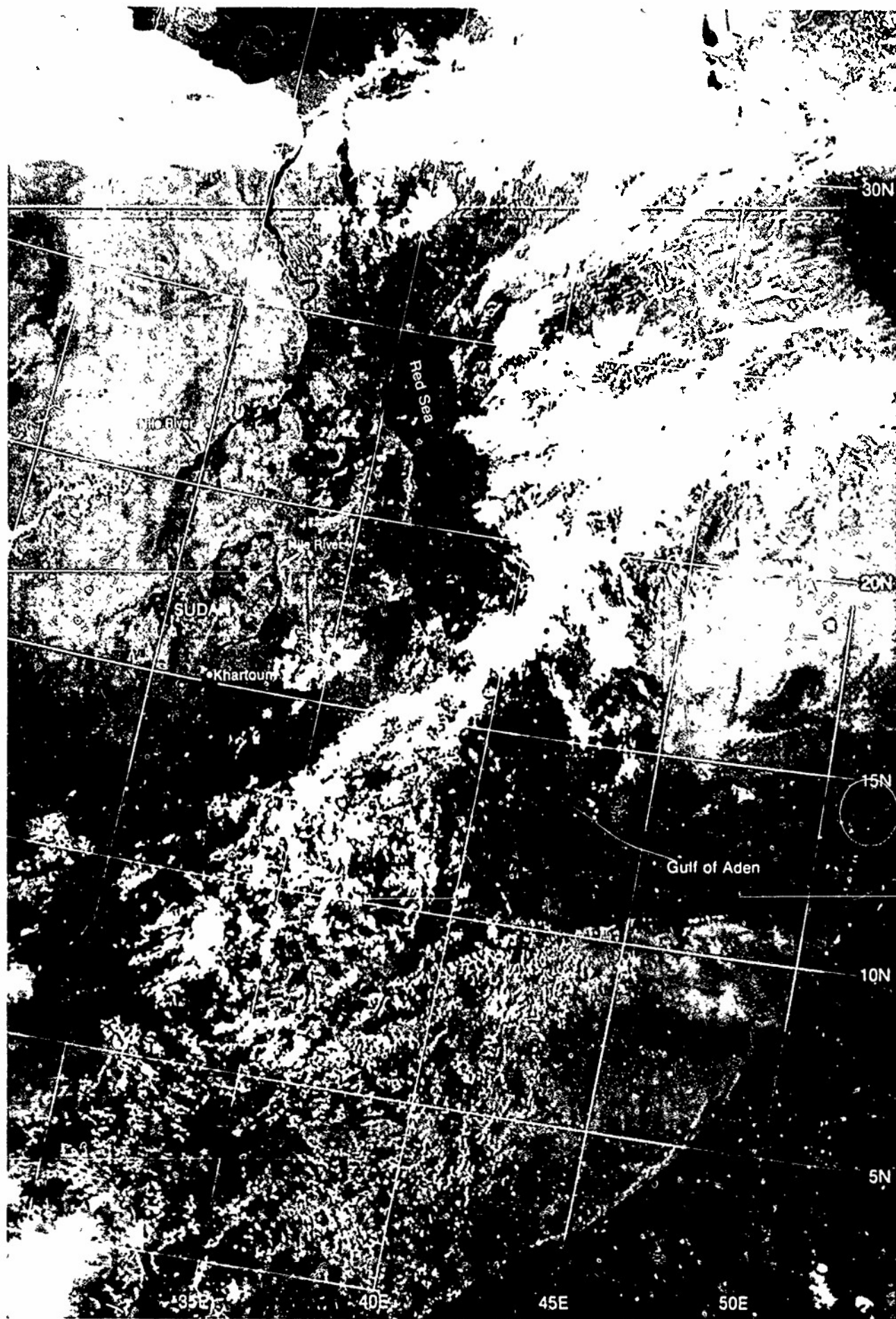
11-9a 1-1 DMSP 1 S Low Enhancement 0823 GMT 4 May 1979
