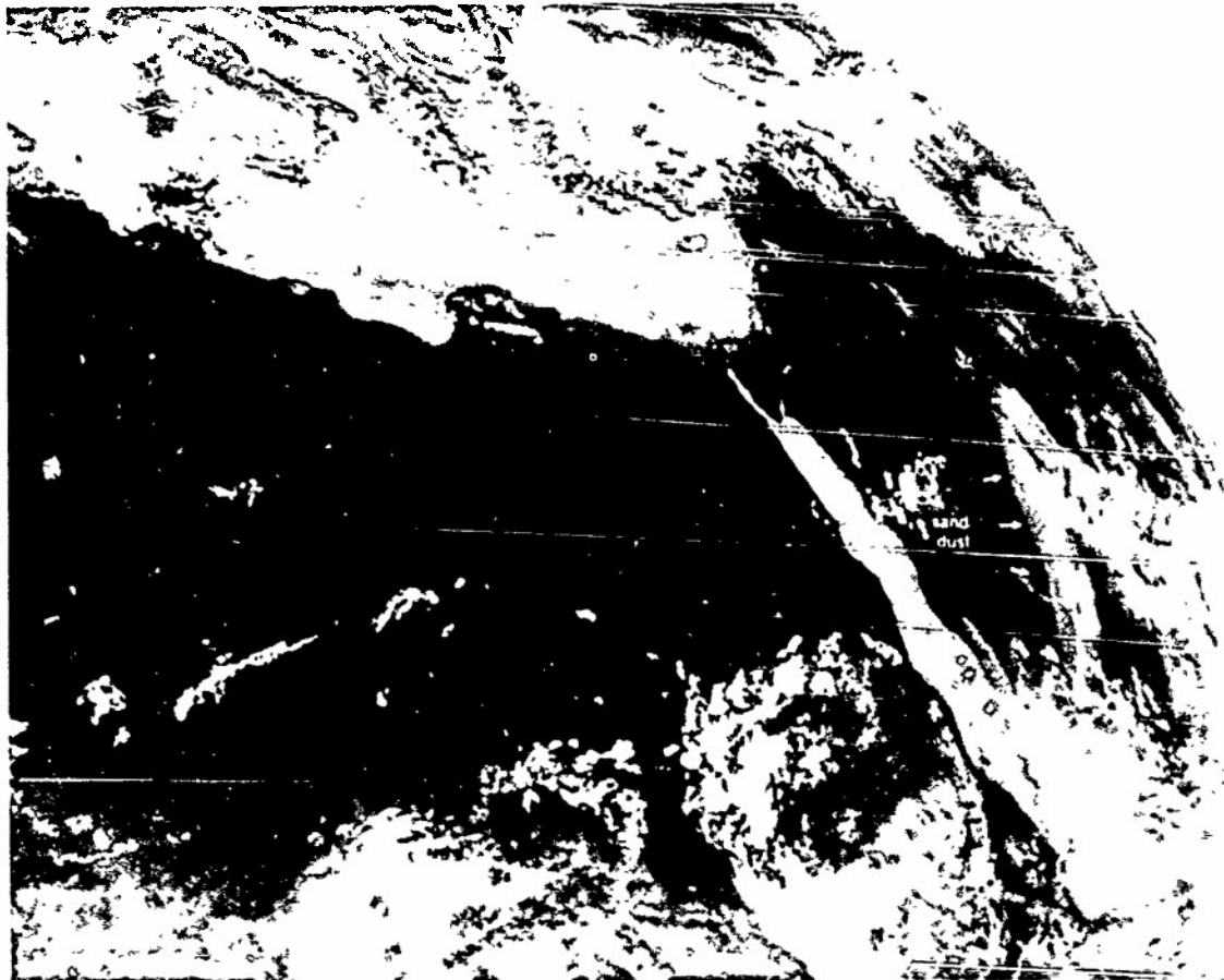
ME-37b. METEOSAT, Enlarged View Infrared Picture 1155 GMT 26 June 1979
