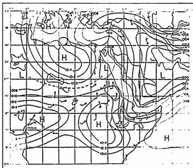
11-1a Typical summer Surface Analysis 0600 GMT 26 July 1943 (Solot, 1950)
