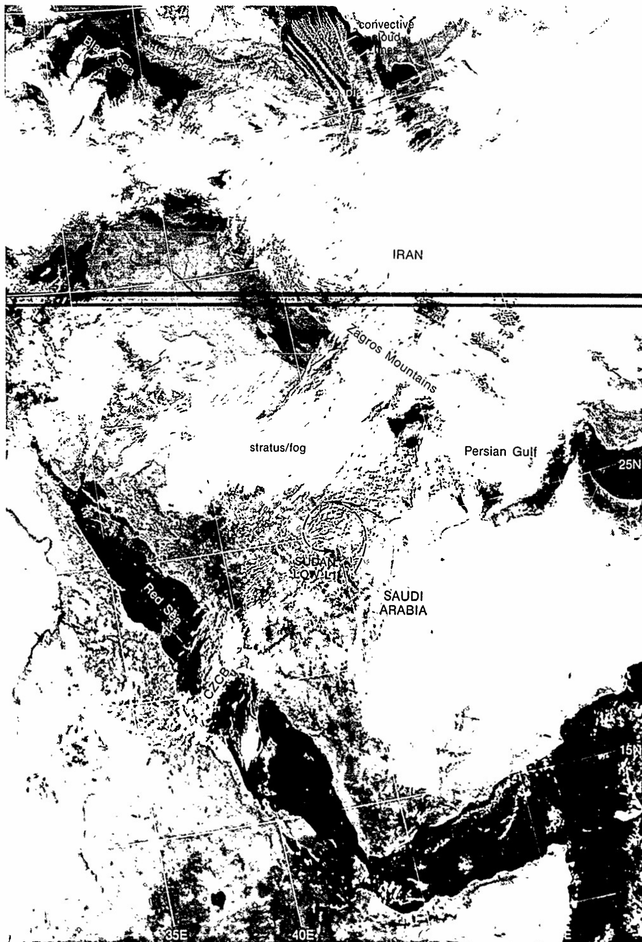
IC-23a 1-4 DMSP L1 Log Enhancement 0712 GMT 23 January 1980. (Note this picture is a repeat of IC-19a.)
