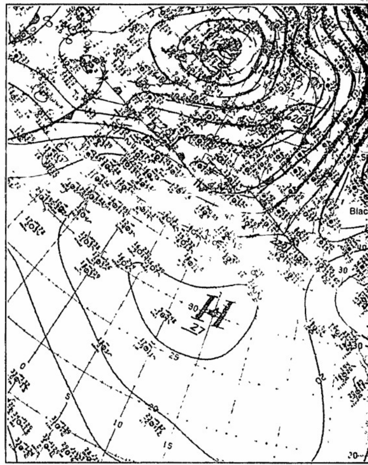
IC-22a. NMC Surface Analysis. 1200 GMT 23 January 1980.
