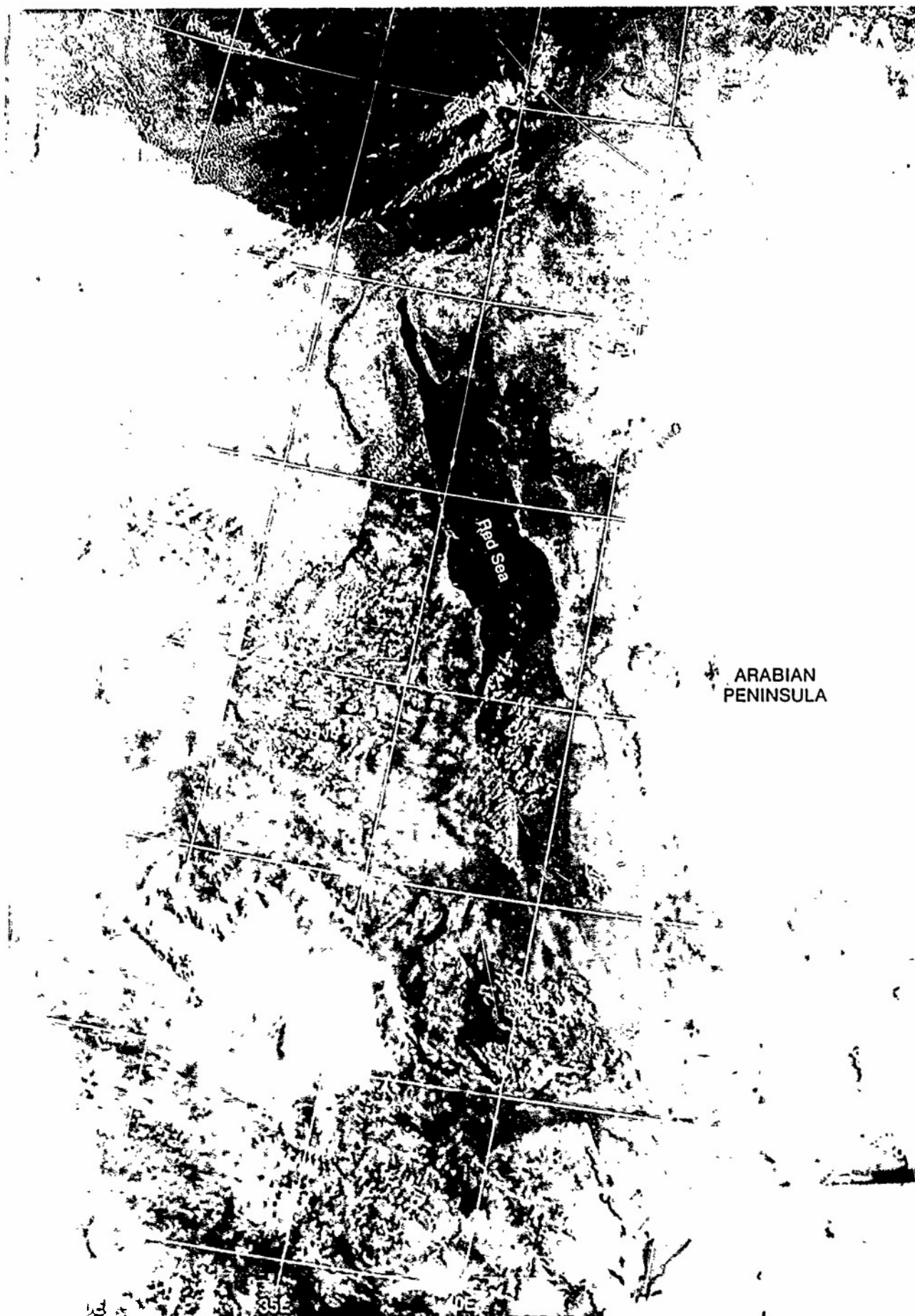
1E-31a 1-3 DMSP 11-1 Low Enhancement 0352 GMT 24 June 1979
