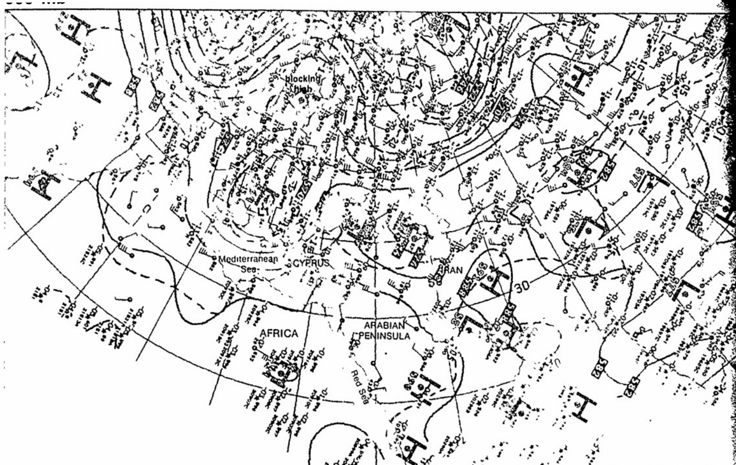
1E-20a NMC 500-mb Analysis 1200 GMT 21 June 1979
