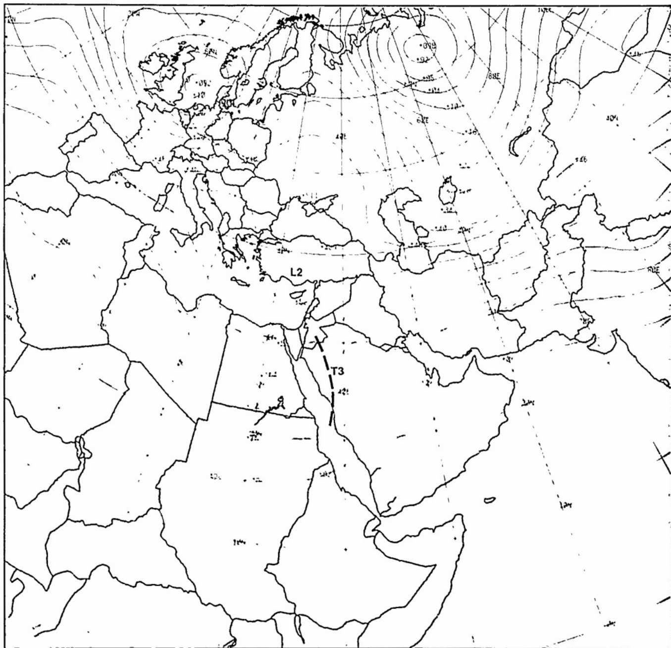
IC-17a FNOG PF 36-hr 500-mb Prognosis Valid 1200 GMT 23 January 1980.
