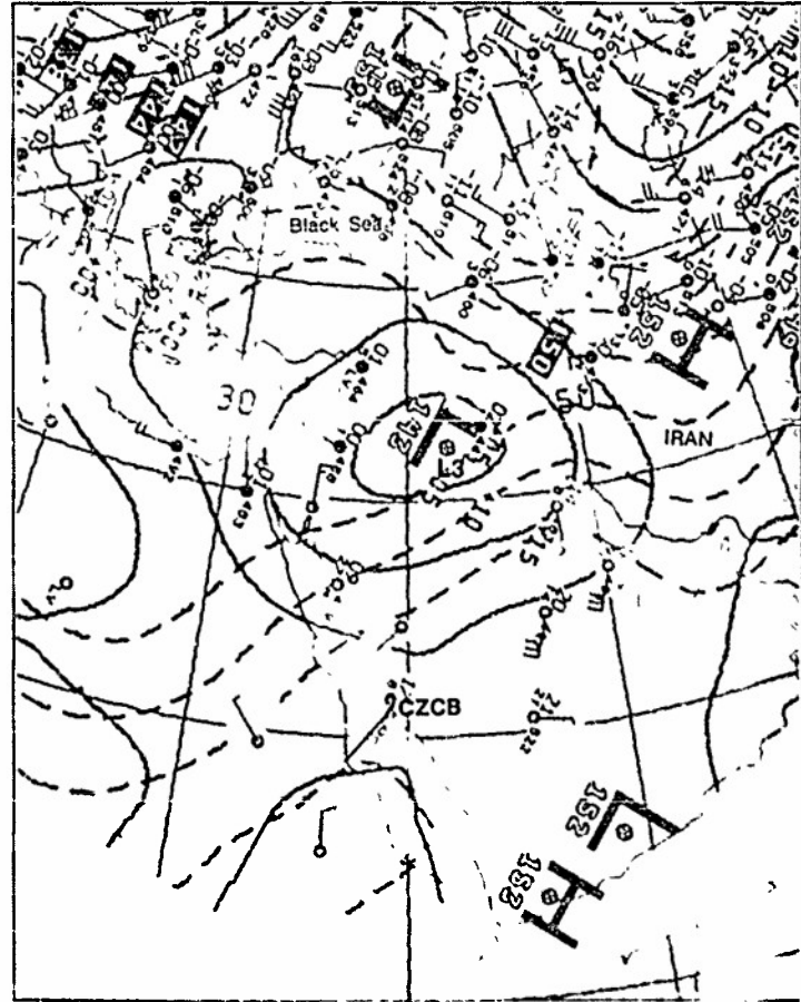
IC-22b. NMC 850-mb Analysis. 0000 GMT 23 January 1980.
