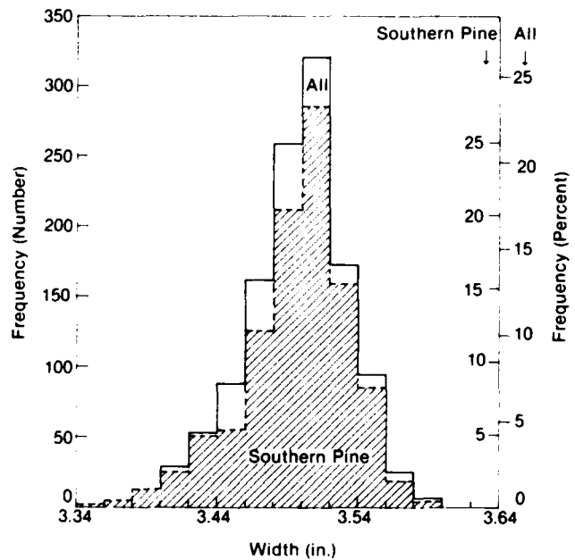
Figure 2.—Distribution of lumber width. (M152112)
