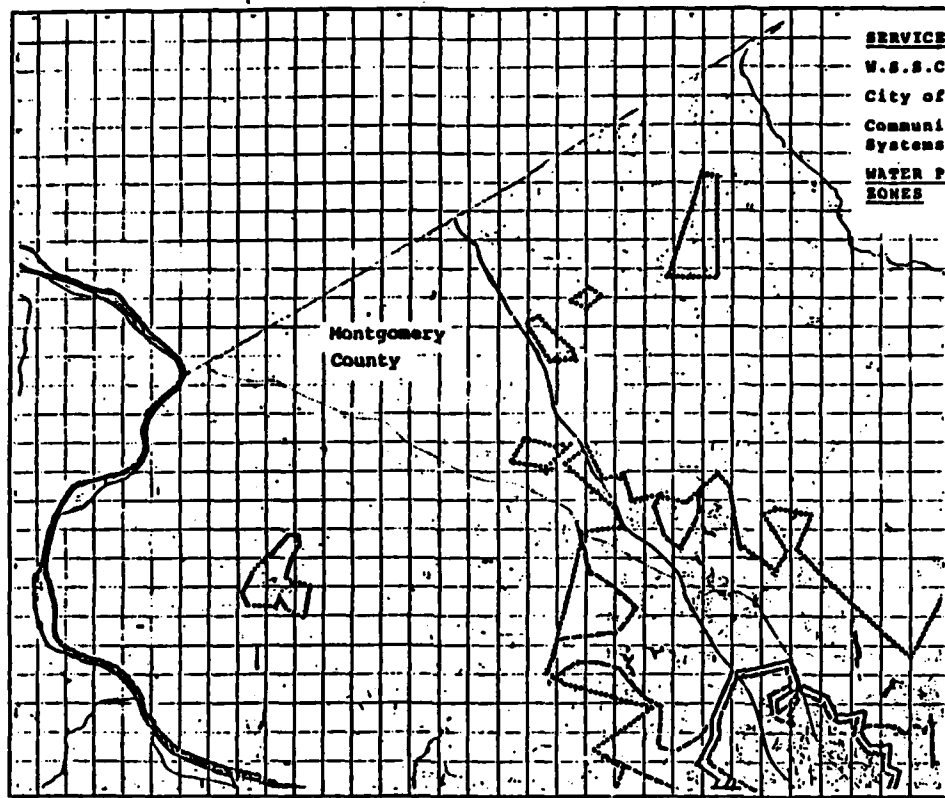
WASHINGTON METROPOLITAN AREA AS OF JANUARY 1, 1970 (BASED ON 1968 DATA) Water Supply Service Areas and Pressure Zones
