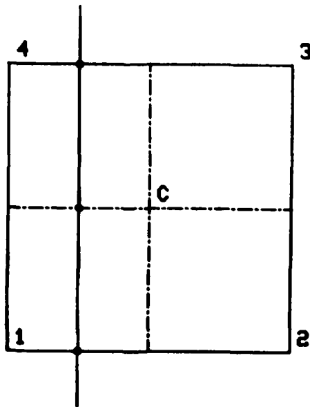
Figure 11. Grid system for TYPE = 3, NNELE = 4, and for all TYPE values for NNELE = 8
