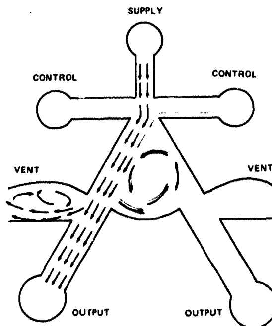
Figure 8. Wall-attachment fluidic bistable amplifier.
