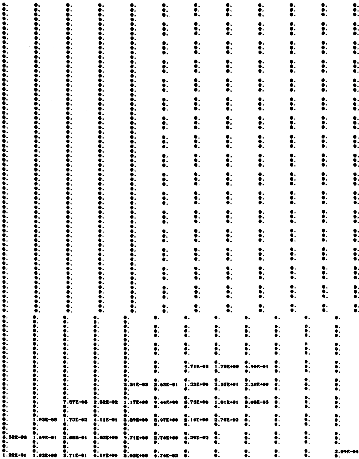
Figure D-5. Common input file XE133.LLNL - 40 × 40 doses due to ^{133}\text{Xe} each time step.
