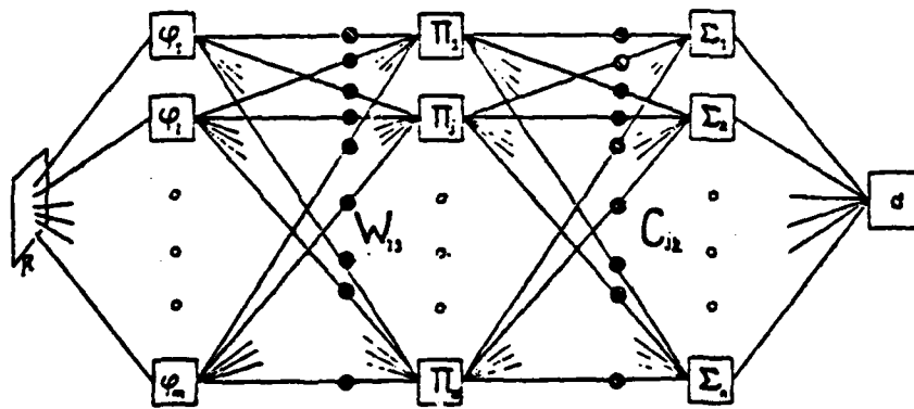
Fig. 7.30. A multilayer perceptron capable of making decisions ( d ). (From Minsky and Papert [672].) The adaptations controlling \Delta w_{ij} and \Delta C_{jk} might benefit from feedback of information concerning the system state.
