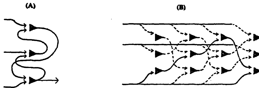
Fig. 7.29. Different connection matrices. Are those in (A) equivalent to those darkened in (B)? (There is feedback in A.) Are some elements and connections in B superfluous? (Even if different transfer functions of several elements could be combined, the connections would allow unique dependencies between inputs, elements, and outputs). (Sketches after Minsky and Papert [672].)
