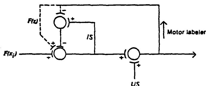
Fig. 7.10. Schema for motor (M) labeled reinforcements derived from Uttley's informon model. The US activates neurons which act directly (or indirectly) as the F(z) input. Selective labeling of the "upstream" neurons which project, selectively, to the activated units is potentiated because of positive feedback within the circuitry. For this schema to operate successfully, some feature such as local recurrent inhibition would be required to monitor the system state and prevent explosive buildup from the positive feedback. IS=feedback of information concerning internal system state.
