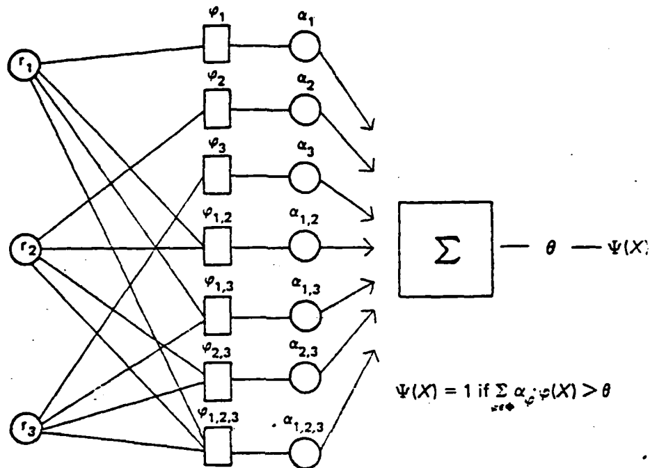
Fig. 7.27. A perceptron reduced to Group Invariance Theorem coefficients. (From Minsky and Papert [672].)
