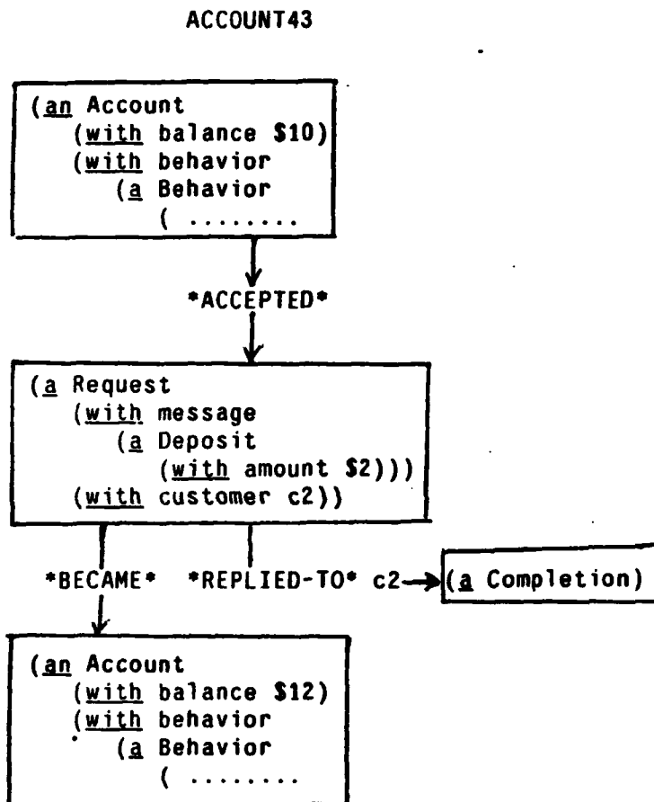
Figure 2-1: A Happening
