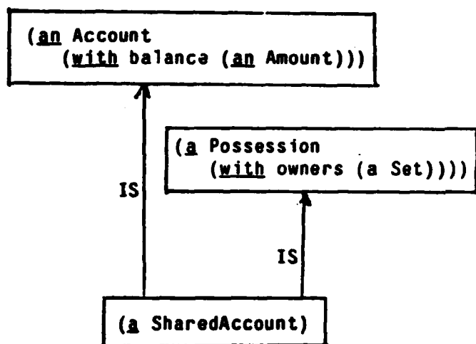
Figure 2-2: Multiple Inheritance
