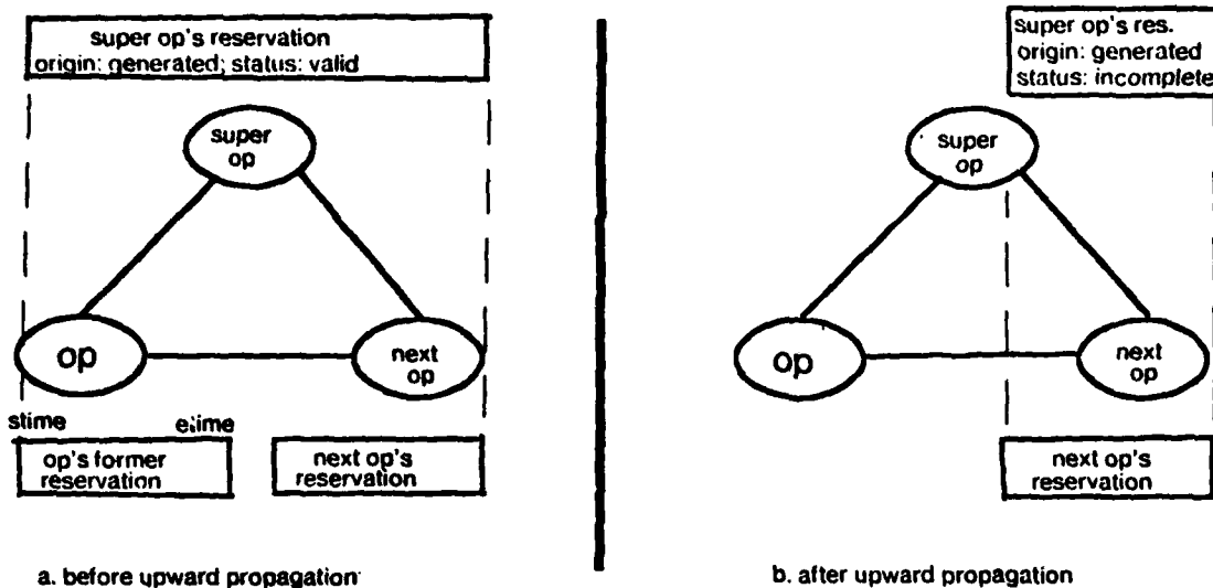
Figure 5-18: Adjusting the scope of a previously generated parent reservation to reflect the removal of op 's reservation
