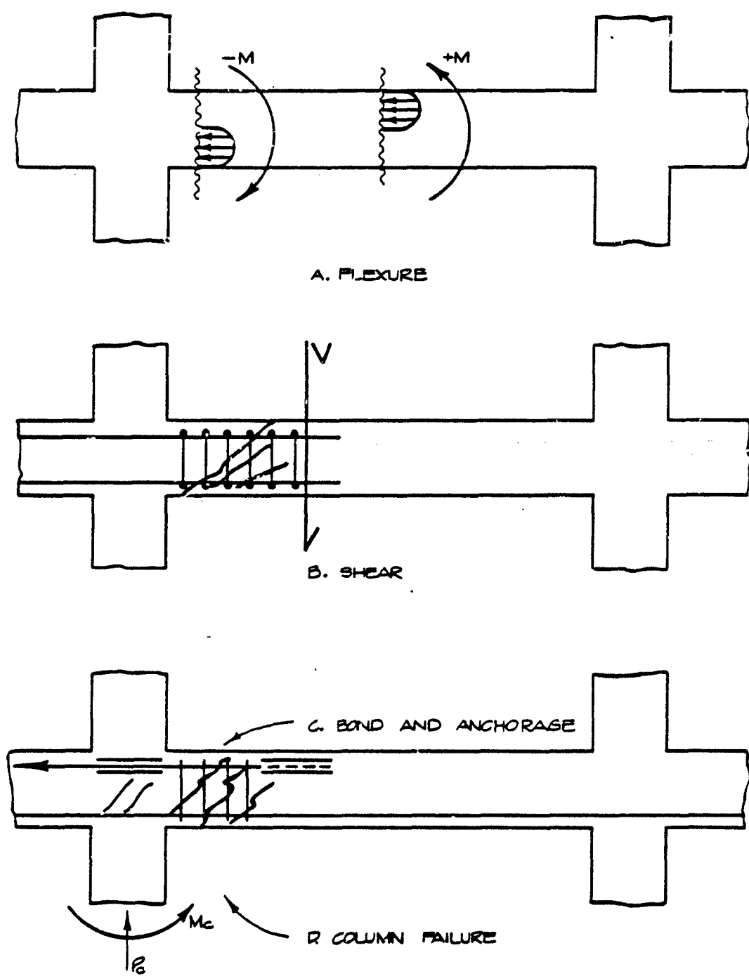
Fig. 5. Failure Modes for the Two-Way Slab System.
