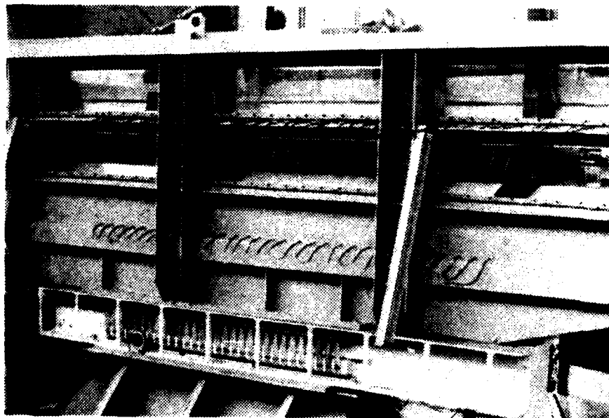
Fig. 3b. Cascade Test Section, Steel Wall Installed
