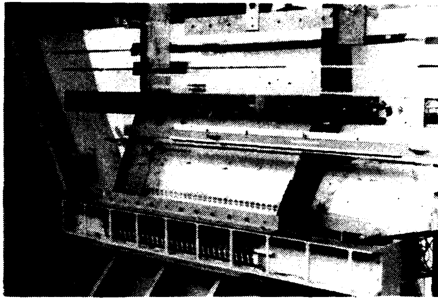
Fig. 3a. Cascade Test Section, Plexiglass Wall Installed
