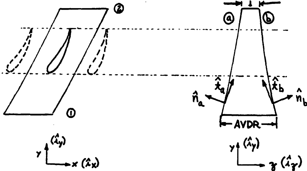
Figure C.1. Blade Space Control Volume
