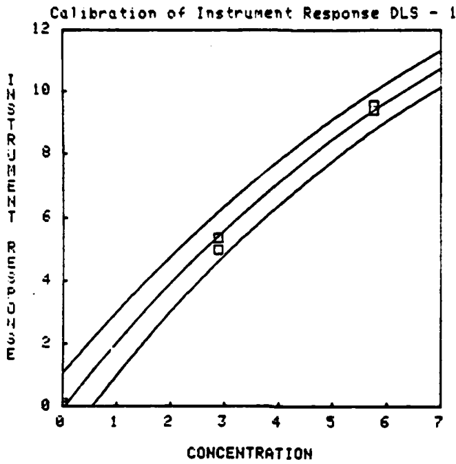
Calibration Curve # 2
