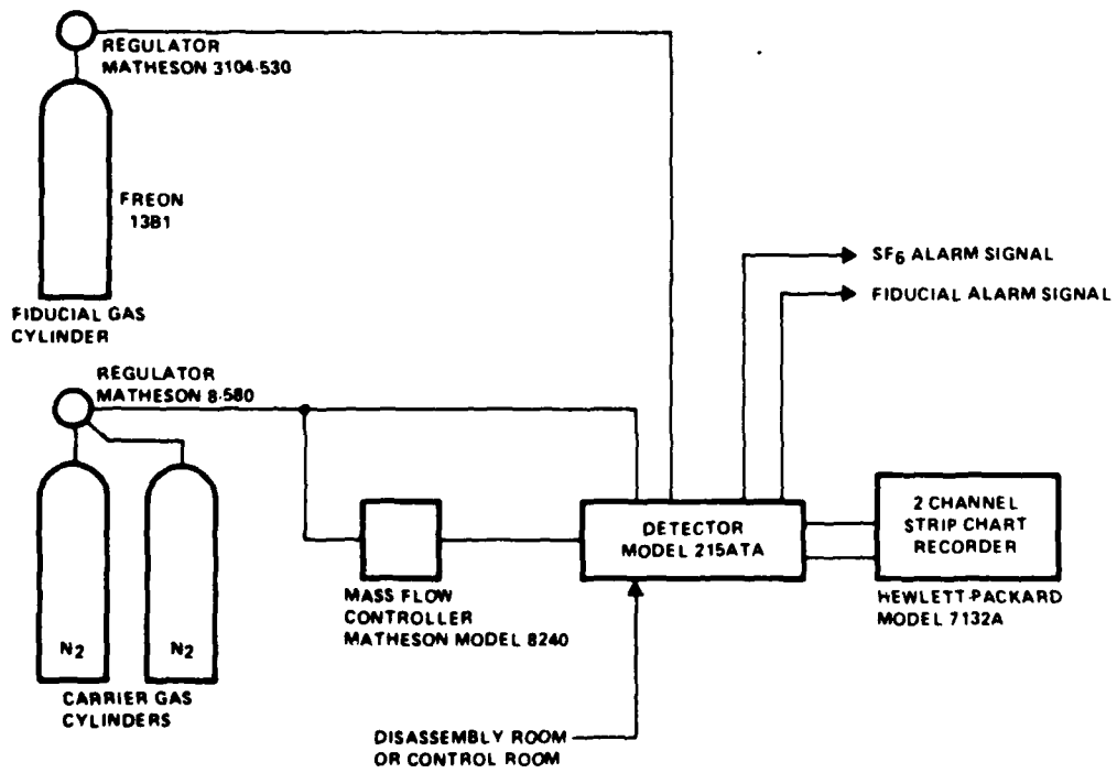
Figure 13 SF 6 FLOW DIAGRAM
