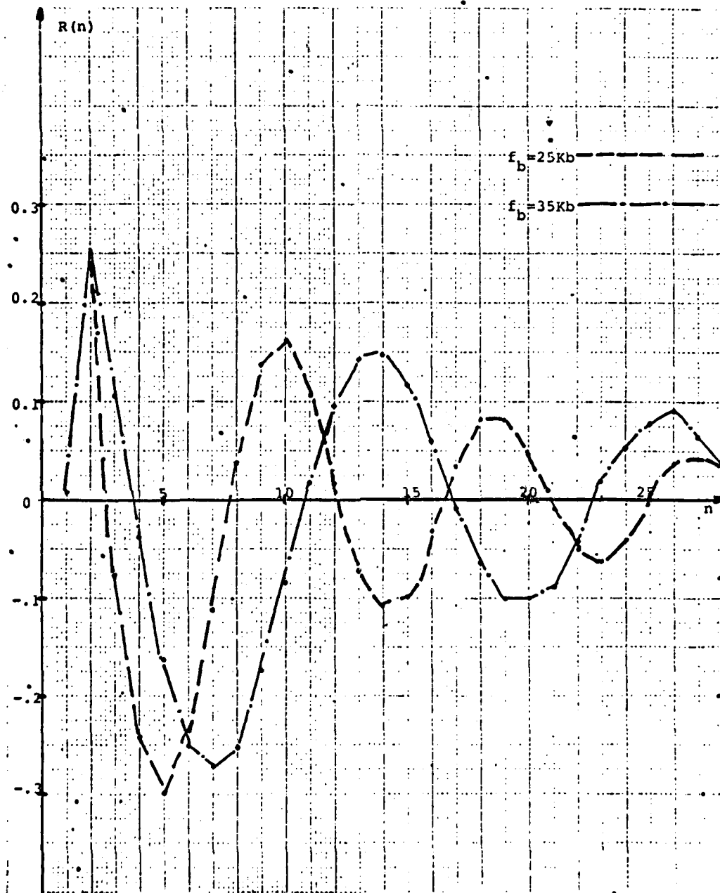
Figure 5.5.1 Autocorrelation of DM output of 9600bps modem for various sampling rates
