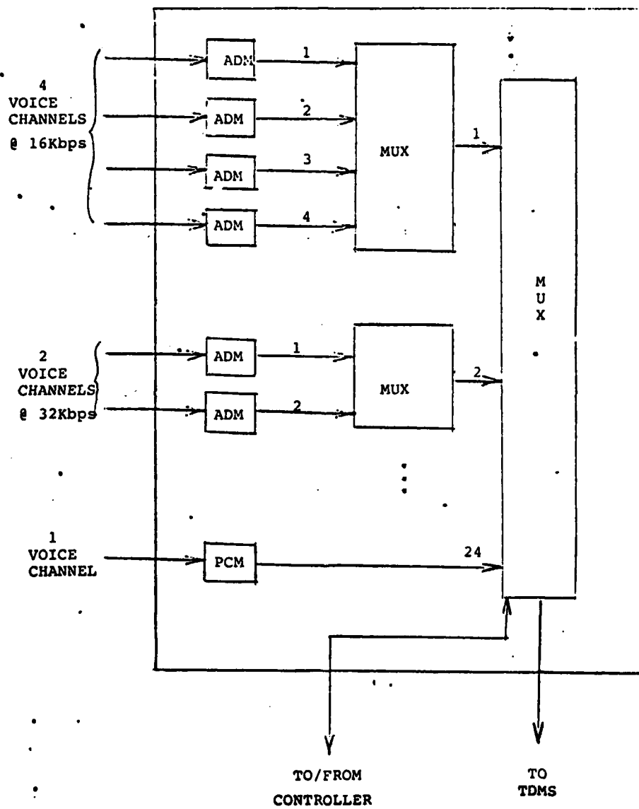
Figure 5.7.2.1 Speech concentrator
