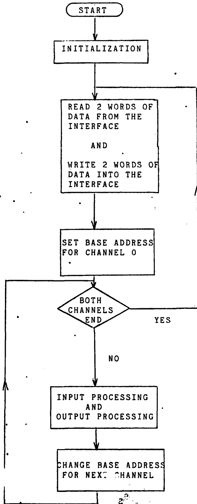
Figure 2.3.2.1 General flow chart of simulator
