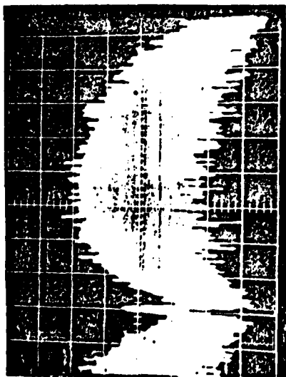
Measured Power Spectral density of 2400 bps duobinary modem (500 Hz/div)
