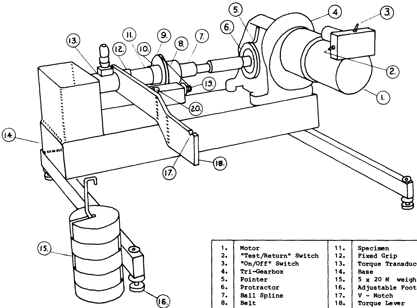
Fig. 1. Torsion testing machine
