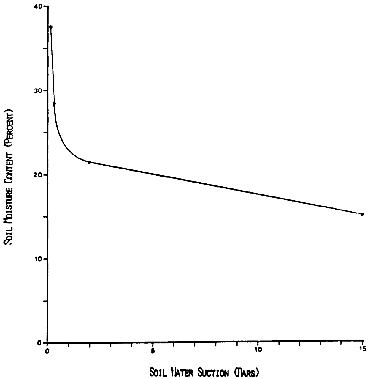
Figure 19. Relationship between soil water suction and percentage moisture retained on clay loam texture (1704-B2)
