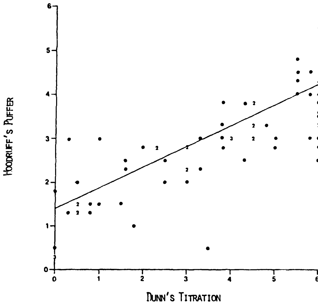
Figure 21. Relationship between Dunn's Titration and Woodruff's Buffer line requirement methods.
