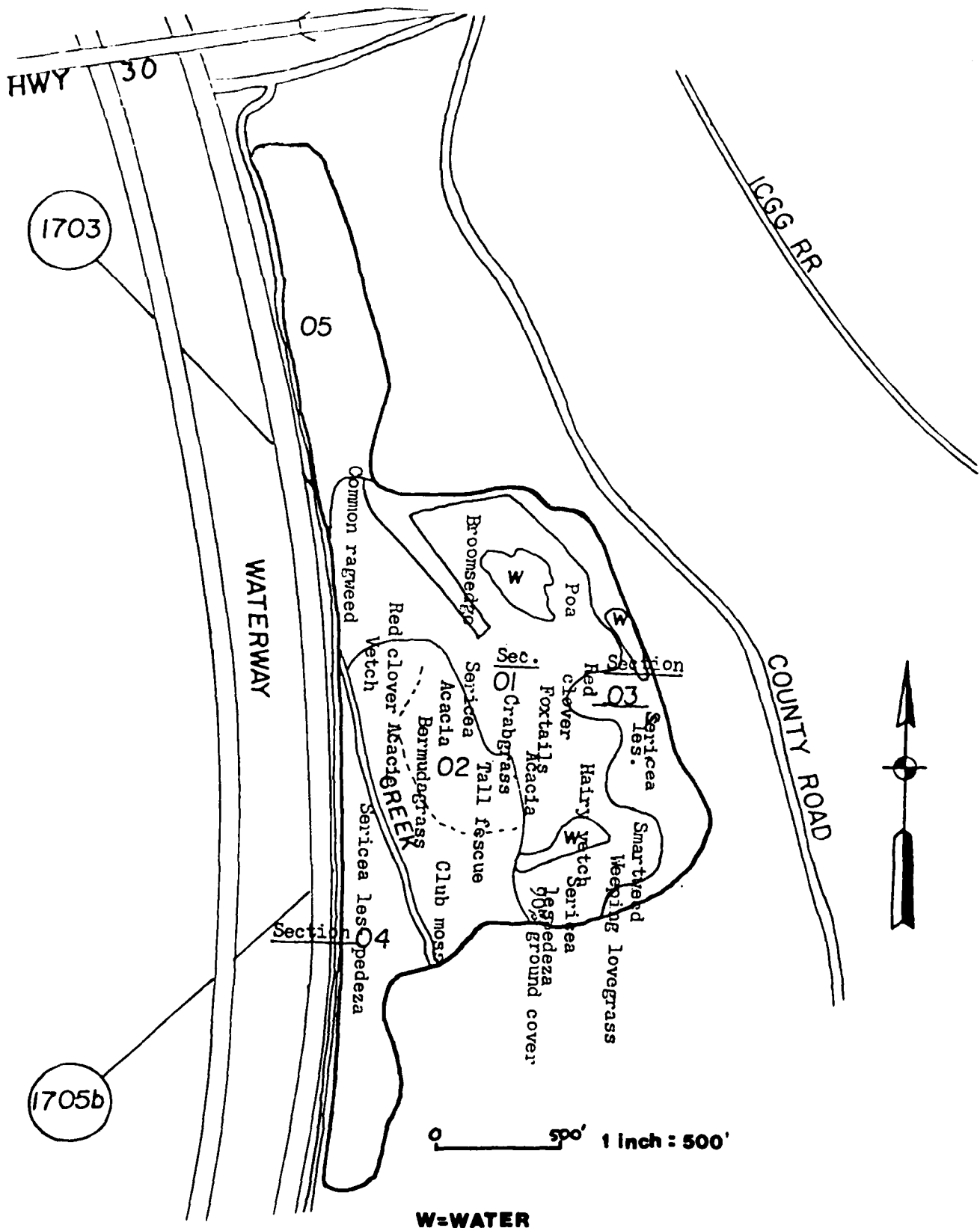
Figure 24. Vegetation evaluation on disposal area 1704, July, 1982.
