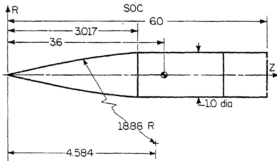
Figure 1 The Geometry of a Six-Caliber Projectile
