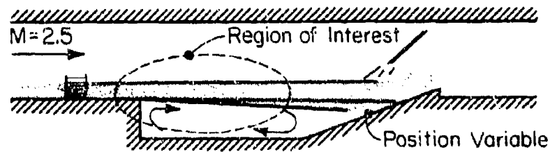
Figure 6(b) Constant pressure shear layer with recirculation.
