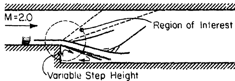
Figure 6(c) Backward-facing step flowfield.
