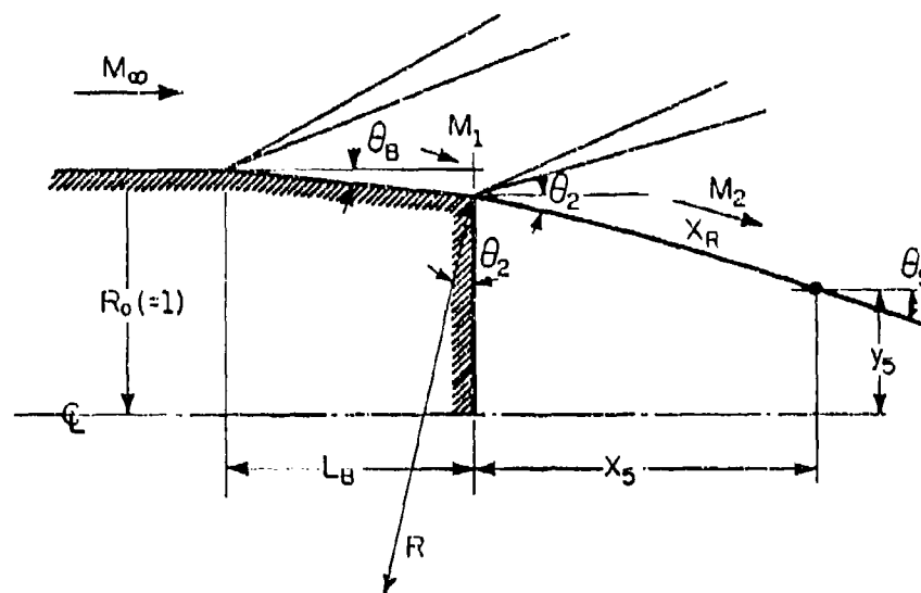
Figure 3 Inviscid External Flow past Boattail and Near Wake (by Method of Sequential Centered Expansions)
