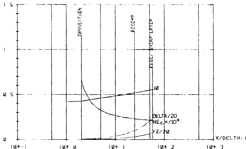
Figure 4 Development of Two-Layer Mixing Profile for Input of Table 1, Solution of Table 2 ("Natural Transition")
