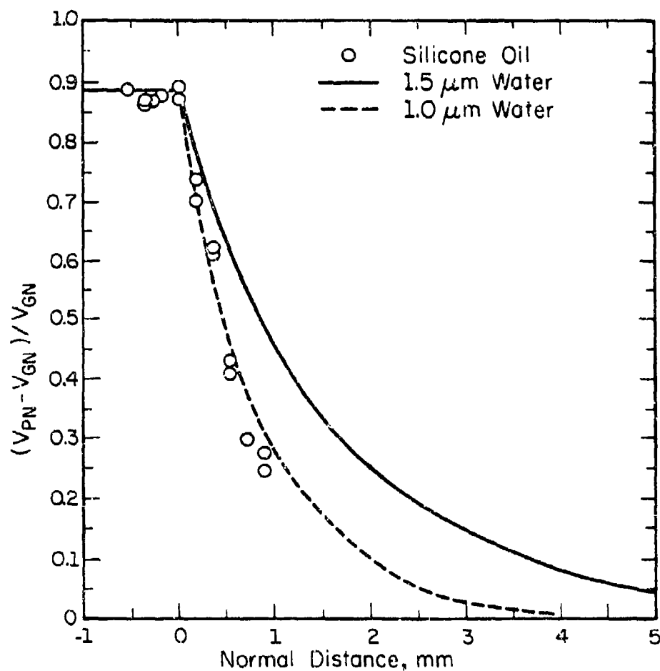
Figure 4 Particle velocity relaxation behind an oblique shock wave at a 15^\circ change in flow direction.
