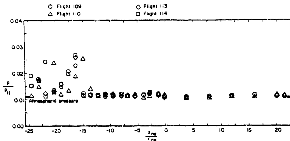
Figure 31. - The pressure history for the PS5 ( x_g = -14.799 r_{ne} ) in the Arrow flight-test program.
