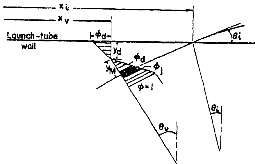
(b) Details of impinging shear-layer for ejector-type flow ( \phi_i > \phi_d , ■ secondary flow)
