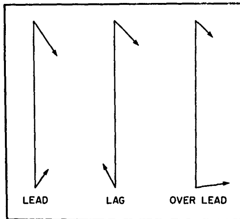
Figure 2. Line-of-sight diagrams showing an example of each of the three tactical geometries used in both experiments. (The lead and lag examples imply relative motion to the right, whereas the overlaid case implies relative motion to the left.)
