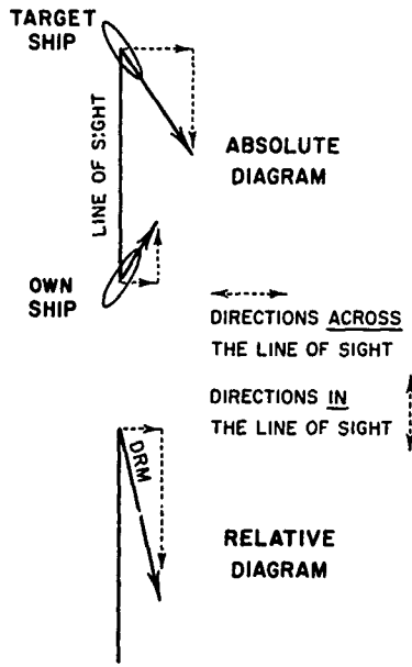
Figure 1. Tactical line-of-sight diagrams. (In the absolute diagram each ship's vector represents its direction and speed with respect to the LOS from own ship to target. The relative diagram is the unique solution representing the target's direction of relative motion with respect to own ship.)
