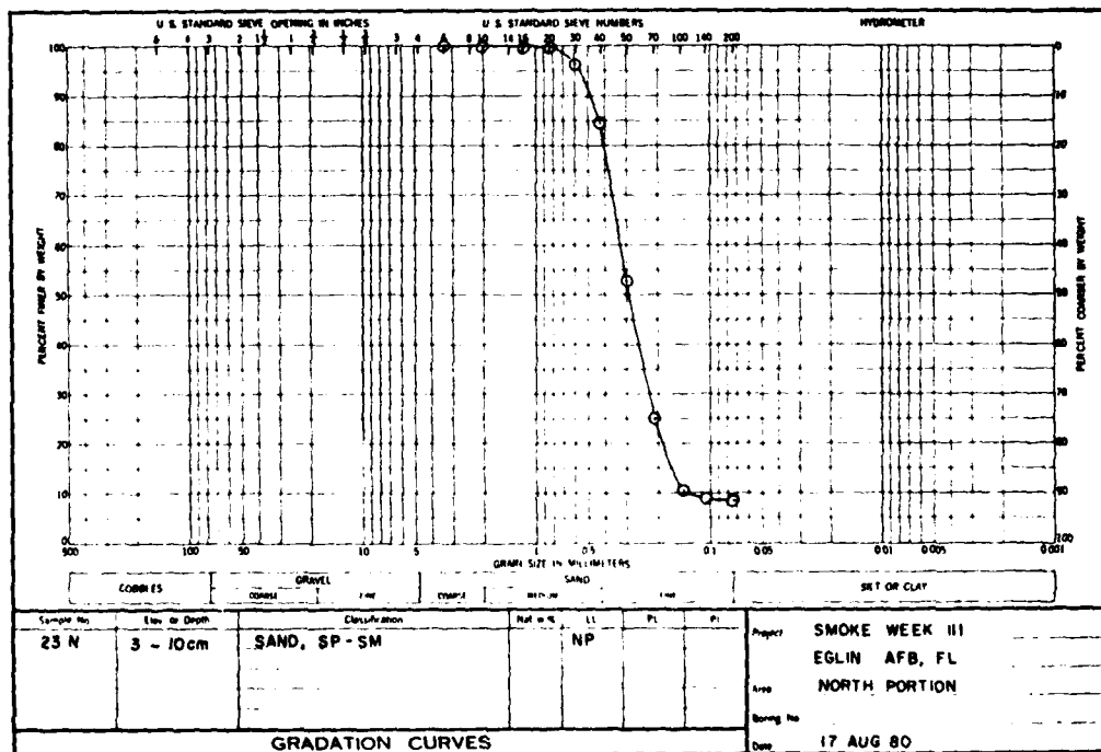
Figure 5. Particle size distribution of sample taken from location 23N
