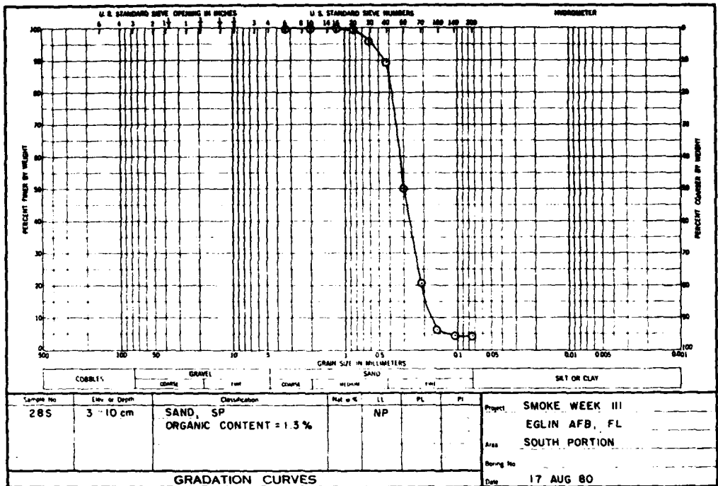
Figure 10. Particle size distribution of sample taken from location 28S
