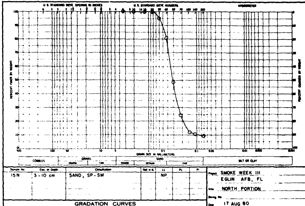
Figure 4. Particle size distribution of sample taken from location 15N
