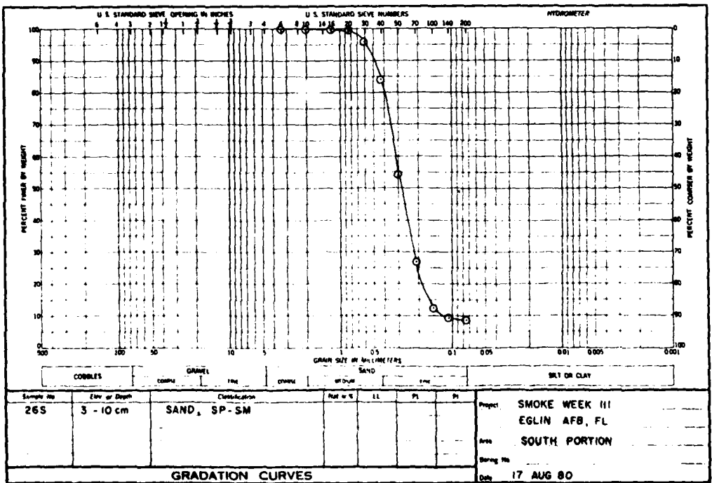
Figure 11. Particle size distribution of sample taken from location 26S
