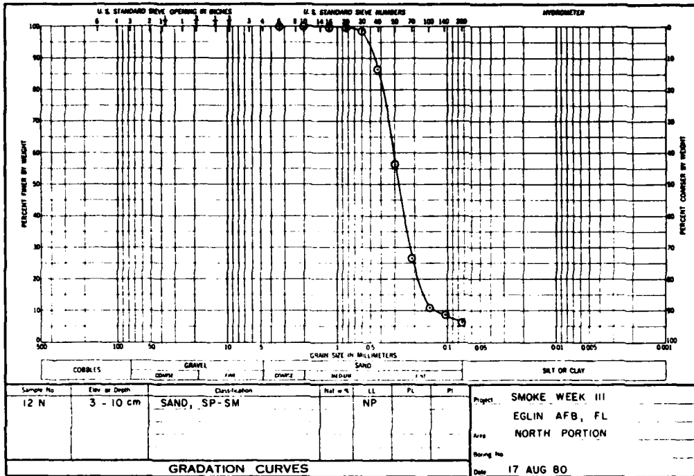
Figure 14. Particle size distribution of sample taken from location 12N
