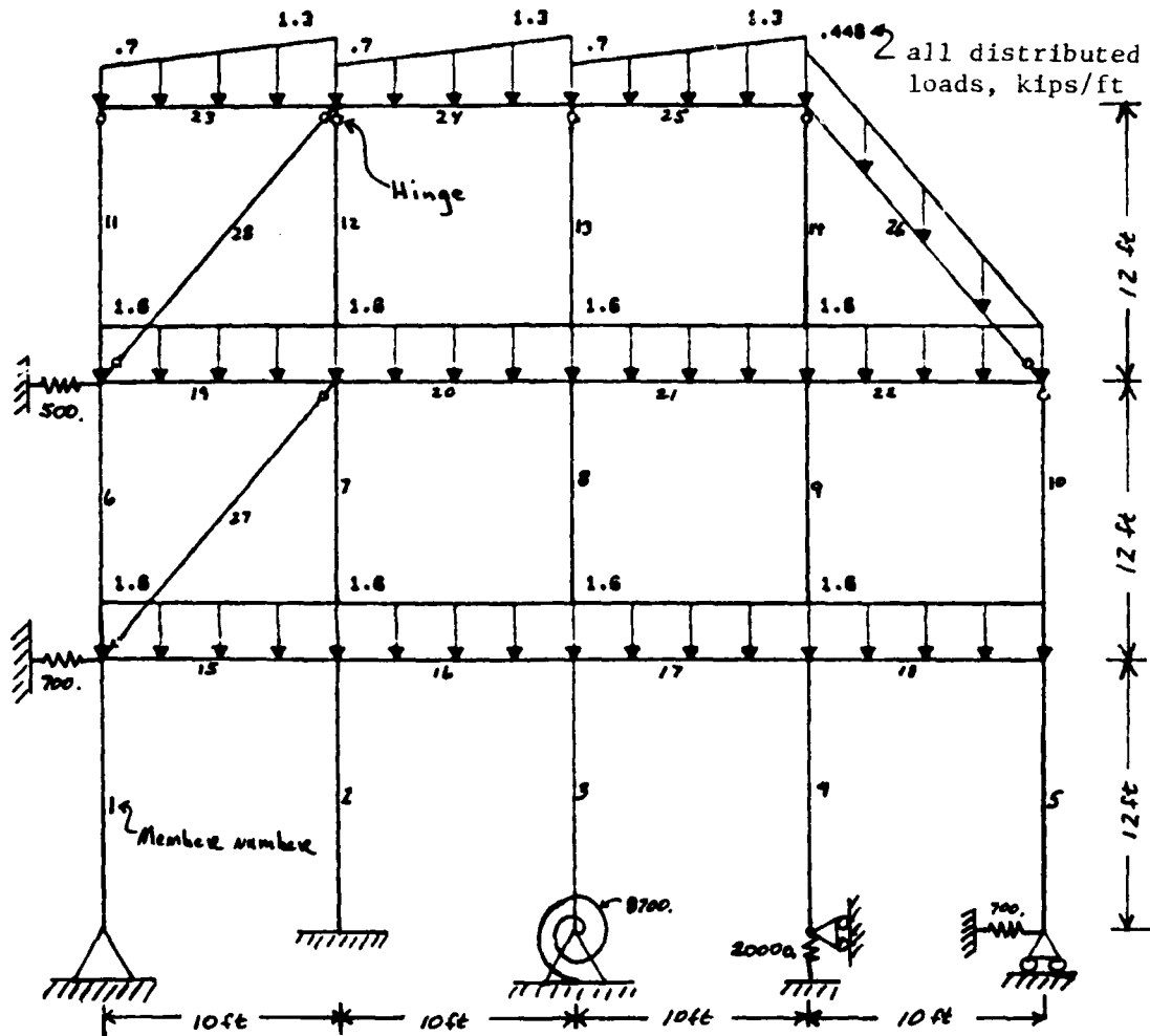
Example Problem 3 - Load Case No. 4
