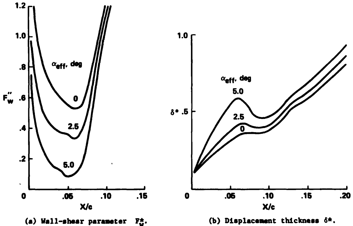
Figure 4.- Variation of wall-shear parameter and displacement thickness with X/c for NACA 0012 airfoil with transition set at X/c = 0.06 ; the effective angle of attack is given by equation (26).
