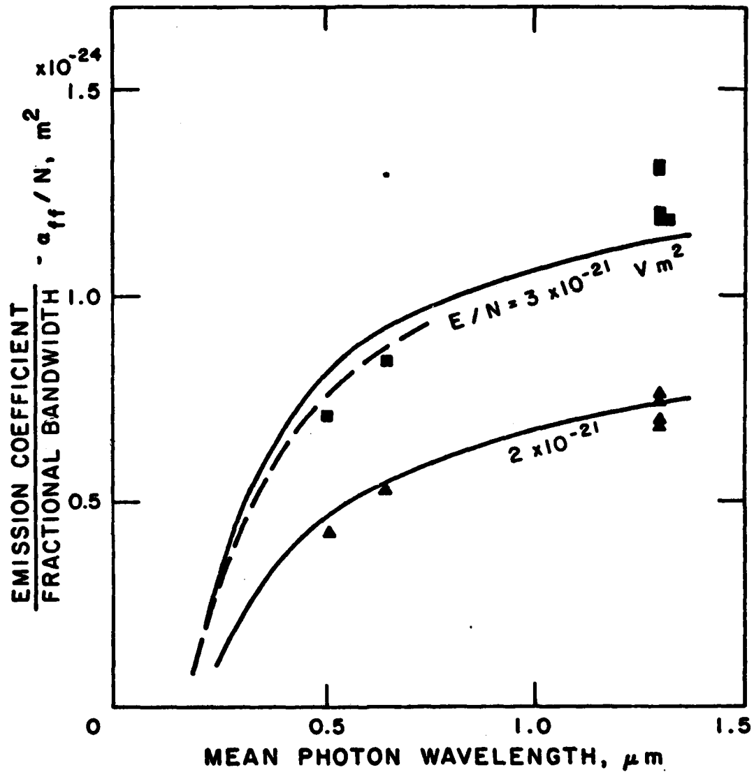
Figure 6. Wavelength dependence of free-free emission coefficient per fractional bandwidth for electrons in Ar. The solid curves are our calculated values, while the dashed curve is from Pfau, Rutscher and Winkler (Reference 22). The triangles and squares are our experimental results for E/N values of 2 and 3 \times 10^{-21} \text{ V m}^2 , respectively.
