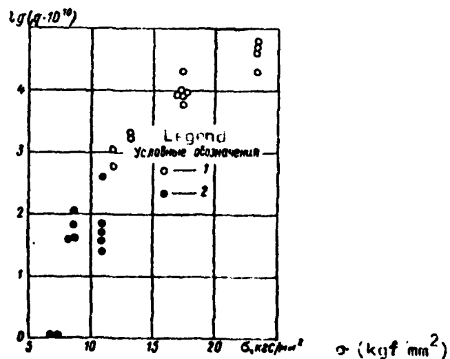
Fig. 2: Specific damage ( q ) vs. amplitude of cyclic bending stress ( \sigma ). 1 - steady conditions; 2 - variable conditions.
