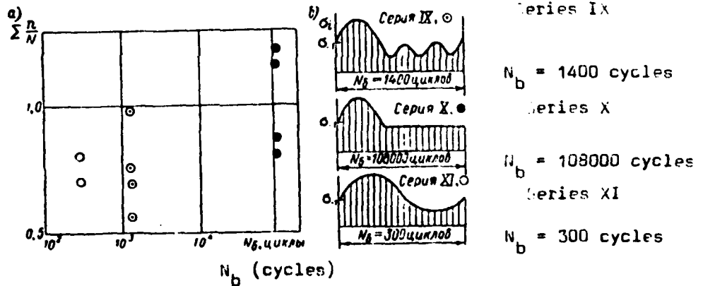
Fig. 4: Influence of the number of cycles in the programmed loading block N_b on the relative durability \sum \frac{p}{N} (a) and the form of the loading blocks (b).
