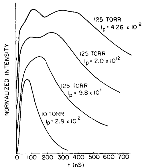
Figure 2. Temporal Profile of the 444.7 nm Line of N^+ . I_p is peak laser intensity in W\ cm^{-2} at the pressures indicated. The 10 torr and first 125 torr curves are generated at I_p of twice threshold for breakdown
