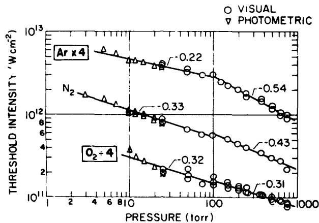
Figure 1. Apparent Breakdown Thresholds for Ar, N 2 and O 2 . Pressure exponents, b , obtained from least squares fits (solid lines) for P > 100 torr and P < 10 torr are indicated. For clarity, the argon and oxygen curves have been offset by a factor of 4 from their actual position
