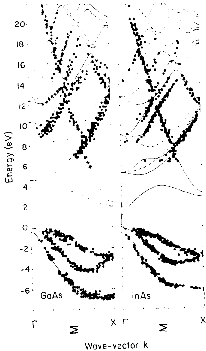
Fig. 1. The comparison of photoemission spectral peaks to the theoretical band by K. Pandey. Each peak gives a conduction and valence band pair of points at a specific value of the wave vector. The spectra were angle-resolved and collected in the direction normal to the (110) cleavage plane.
