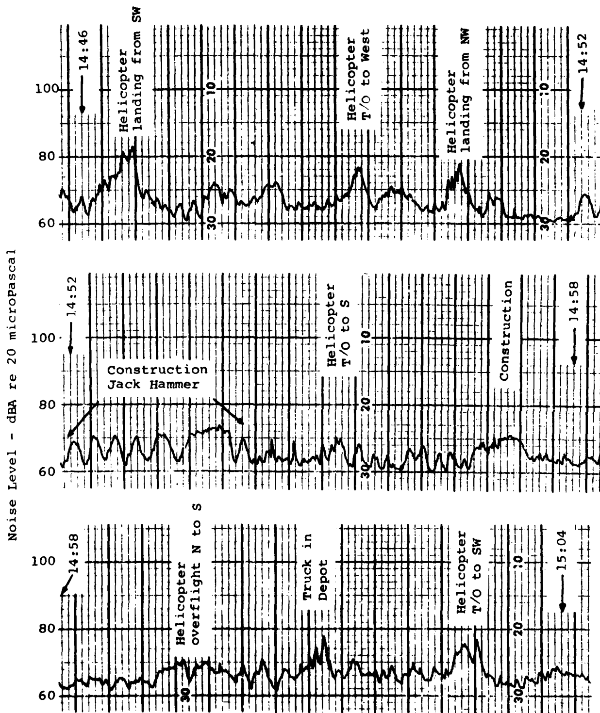
Figure 8. Noise-Level Time History Data - Site No. 1 Vicinity of West 30th Street Heliport New York, New York - November 16, 1982
