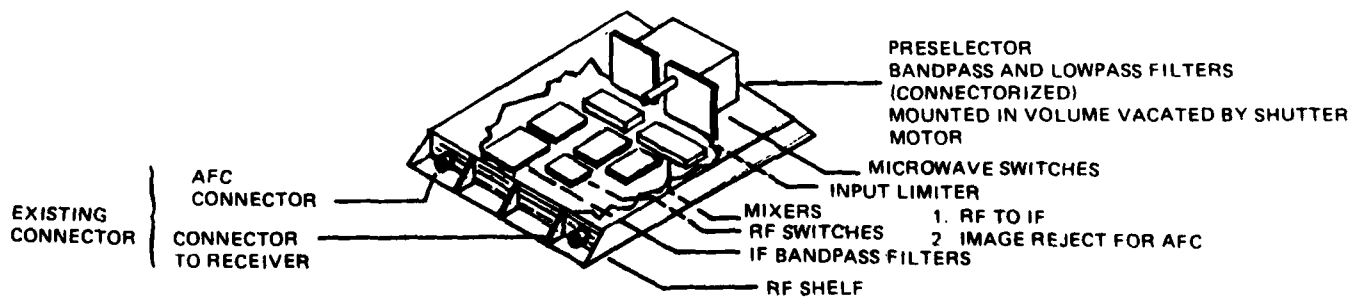
Figure 17 Mechanical configurations of RF sections of SPS-10 receiver as recommended by study.
