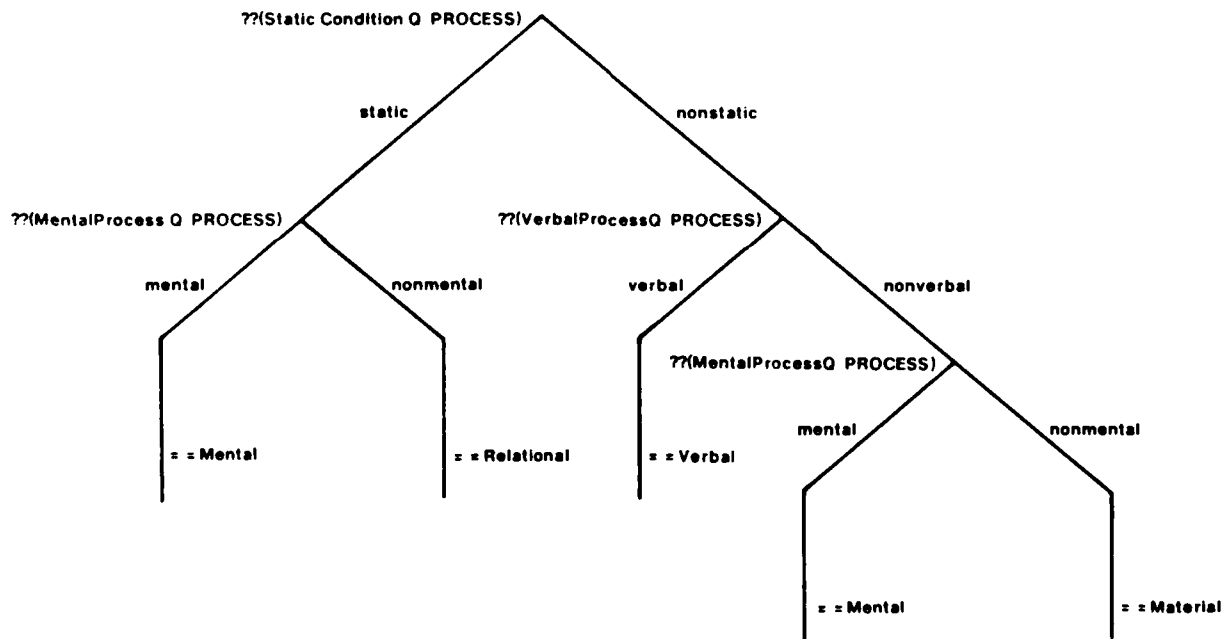
Figure 2-1: The Chooser of the ProcessType system
