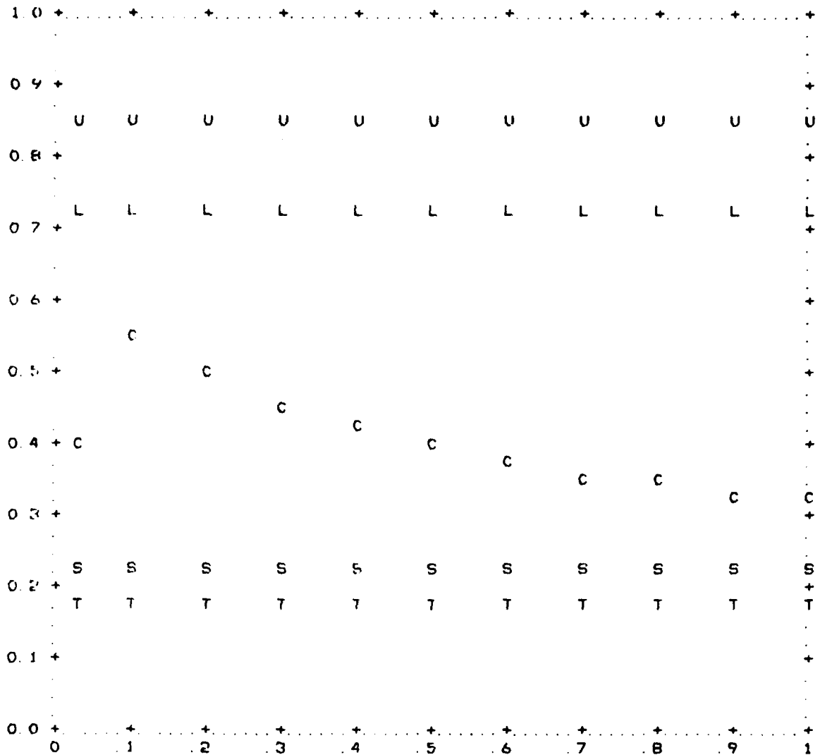
GRAPH OF VAPOR CONCENTRATION AT MAN BREATHING HEIGHT VS DOWNWIND DISTANCE O ORDINATE IS PROPORTIONAL TO LOG(CONCENTRATION) O ABSCISSA IS PROPORTIONAL TO DISTANCE
