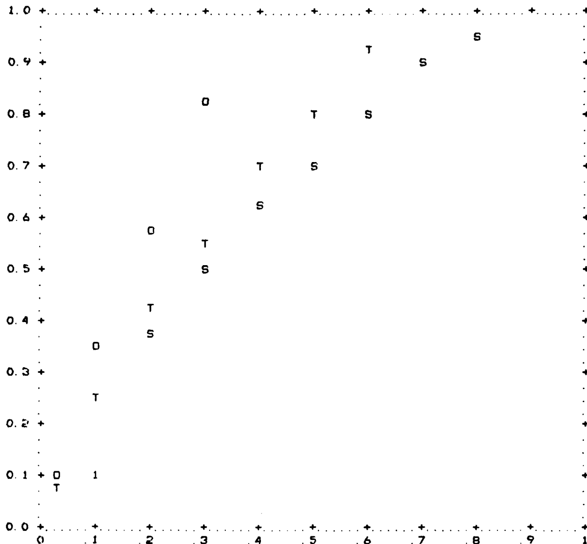
GRAPH OF VAPOR CONCENTRATION CONTOURS AT MAN BREATHING HEIGHT ABOVE THE DECK O ORDINATE IS PROPORTIONAL TO DISTANCE IN THE CROSS-WIND DIRECTION O ABCISSA IS PROPORTIONAL TO DISTANCE IN THE DOWNSTREAM DIRECTION
