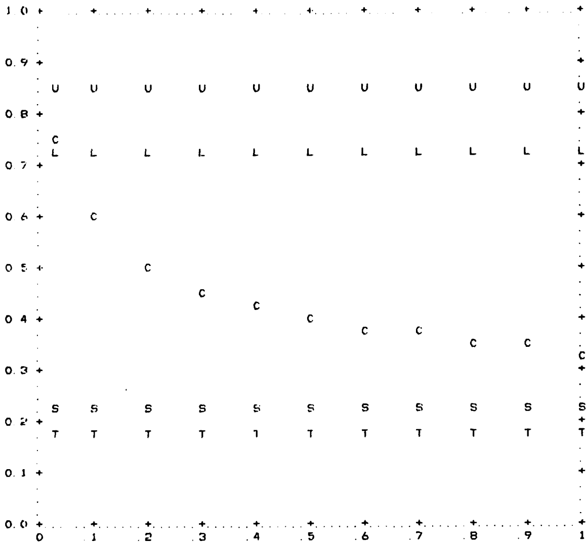
GRAPH OF PLUME CENTERLINE CONCENTRATION VERSUS DOWNWIND DISTANCE O ORDINATE IS PROPORTIONAL TO LOG(CONCENTRATION) O ABSCISSA IS PROPORTIONAL TO DISTANCE
