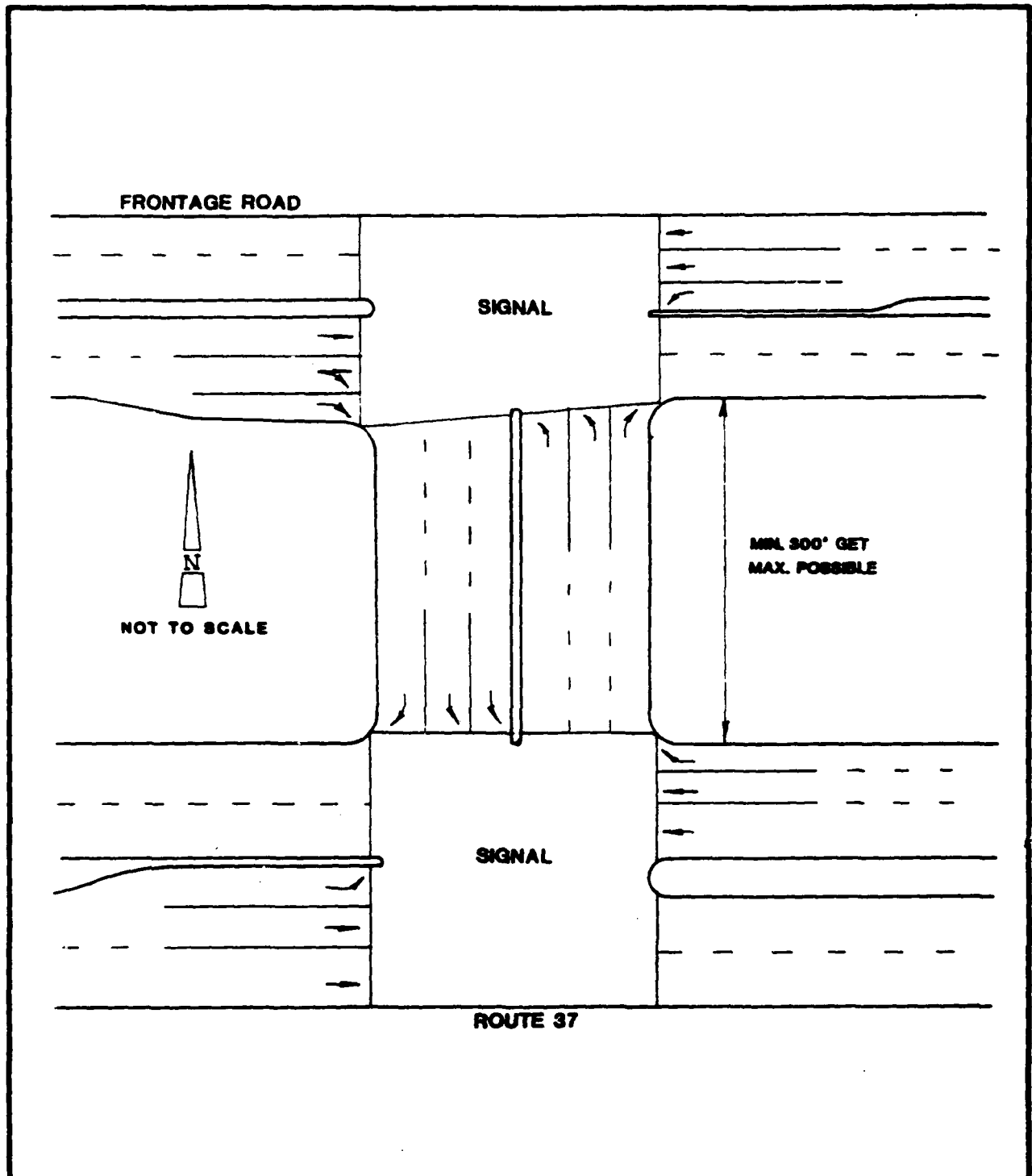
FIGURE IV - 6 INTERSECTION CONFIGURATIONS AT EASTERLY ACCESS POINT
