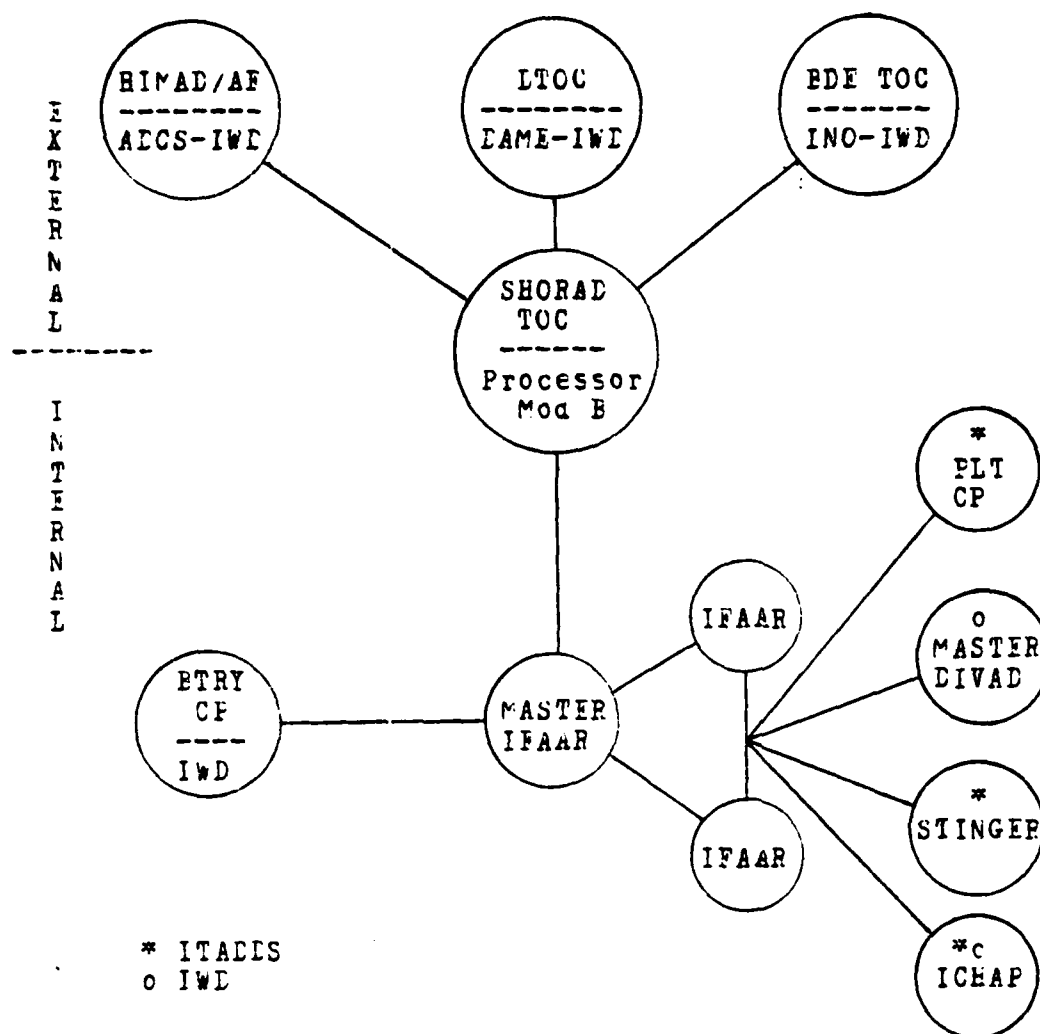
Figure 12. Sanders SHORAD-C2 System Design
