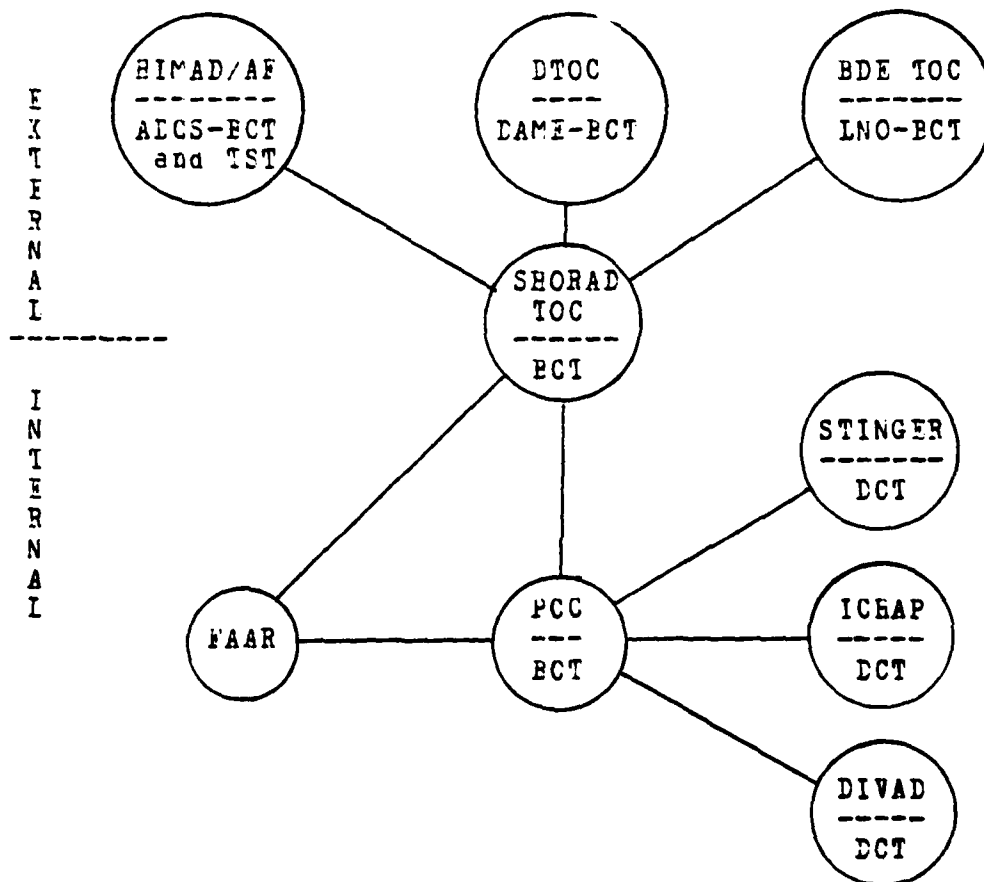
Figure 15. Litton SHORAD-C2 System Design
